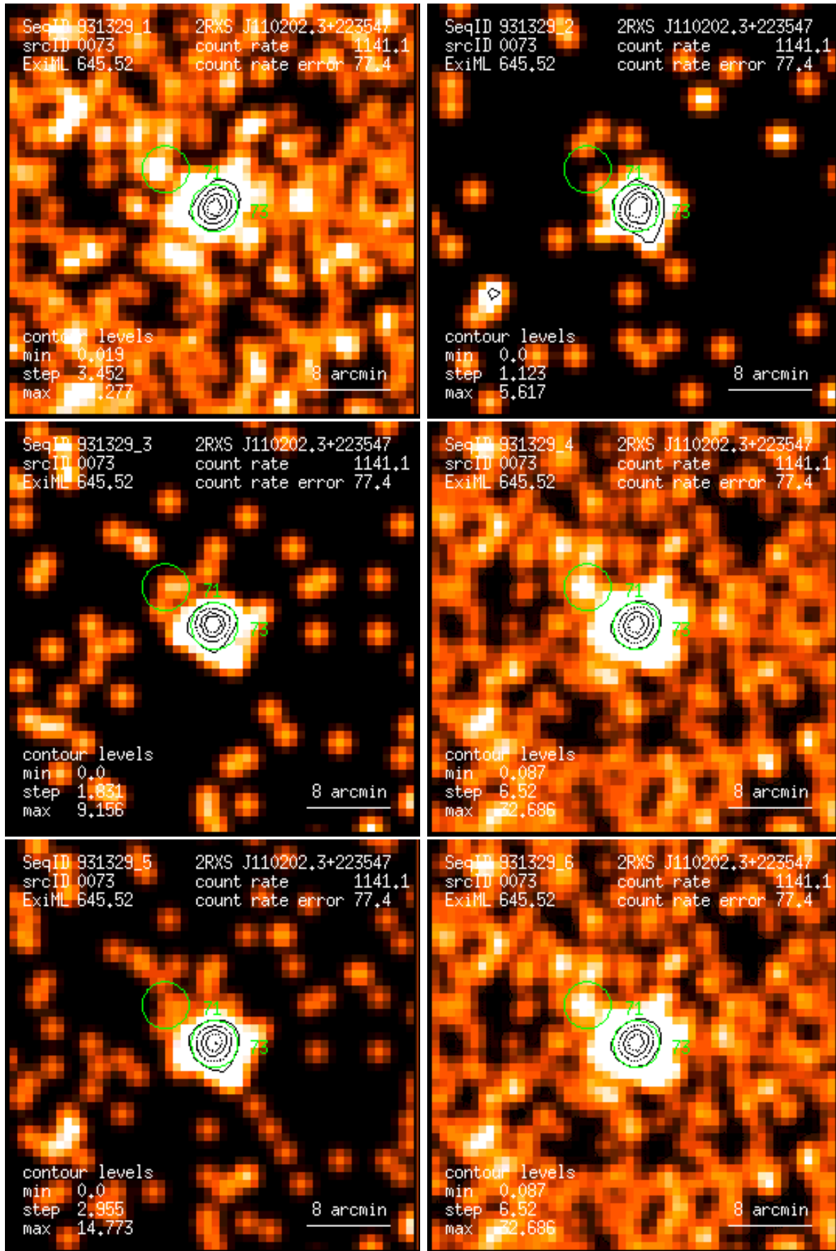
Figure 73: RASS 931329: detection 0073: band rate images, Gaussian filter: (1) PSPC channels 11 – 41, (2) 52 – 90, (3) 91 – 201, (4) 11 – 235, (5) 52 – 201, (6) 11 – 201. Broad band rates in counts/ks. Band rate contour levels in counts/ks/arcmin 2 .
