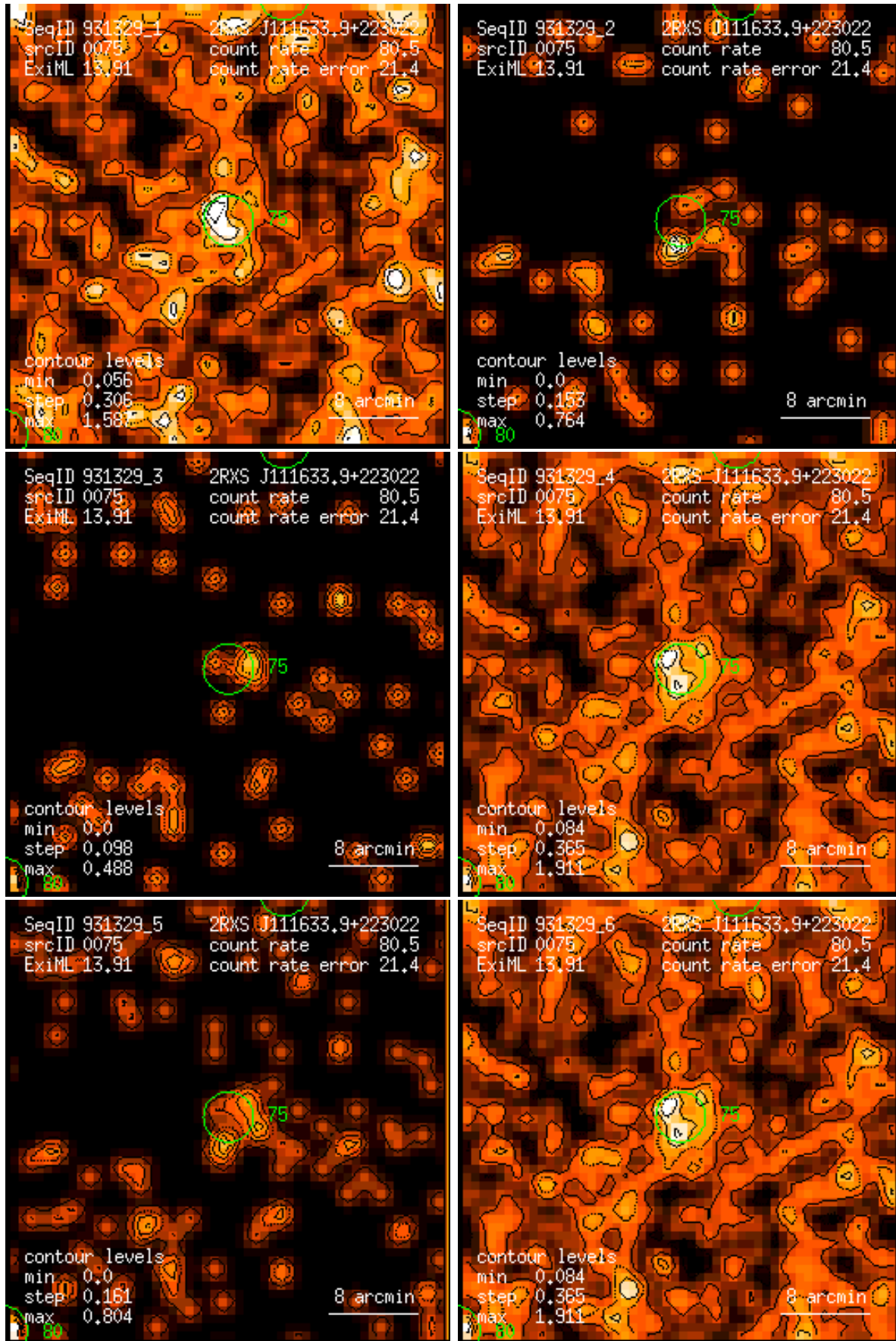
Figure 75: RASS 931329: detection 0075: band rate images, Gaussian filter: (1) PSPC channels 11 – 41, (2) 52 – 90, (3) 91 – 201, (4) 11 – 235, (5) 52 – 201, (6) 11 – 201. Broad band rates in counts/ks. Band rate contour levels in counts/ks/arcmin 2 .
