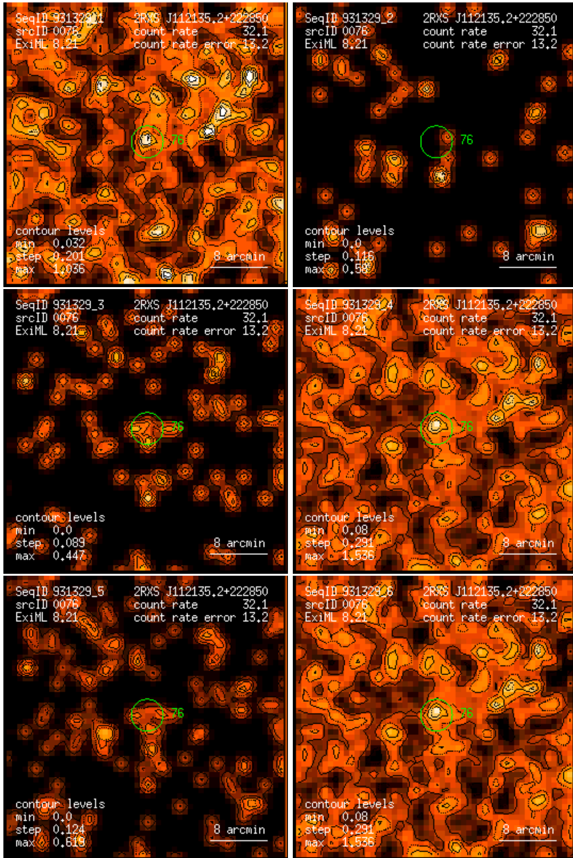
Figure 76: RASS 931329: detection 0076: band rate images, Gaussian filter: (1) PSPC channels 11 – 41, (2) 52 – 90, (3) 91 – 201, (4) 11 – 235, (5) 52 – 201, (6) 11 – 201. Broad band rates in counts/ks. Band rate contour levels in counts/ks/arcmin 2 .
