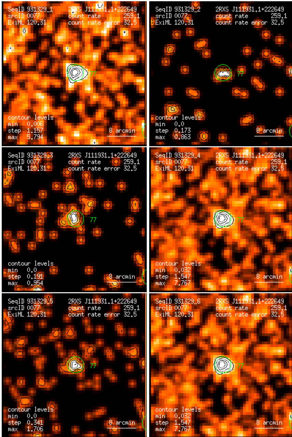
Figure 77: RASS 931329: detection 0077: band rate images, Gaussian filter: (1) PSPC channels 11 – 41, (2) 52 – 90, (3) 91 – 201, (4) 11 – 235, (5) 52 – 201, (6) 11 – 201. Broad band rates in counts/ks. Band rate contour levels in counts/ks/arcmin 2 .
