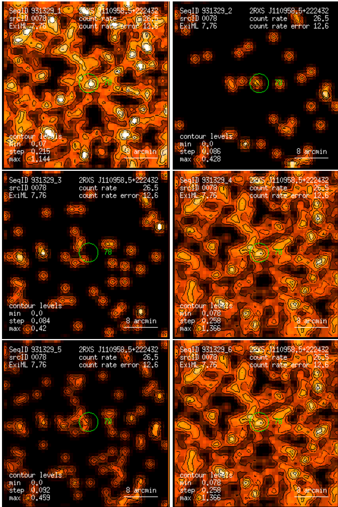
Figure 78: RASS 931329: detection 0078: band rate images, Gaussian filter: (1) PSPC channels 11 – 41, (2) 52 – 90, (3) 91 – 201, (4) 11 – 235, (5) 52 – 201, (6) 11 – 201. Broad band rates in counts/ks. Band rate contour levels in counts/ks/arcmin 2 .
