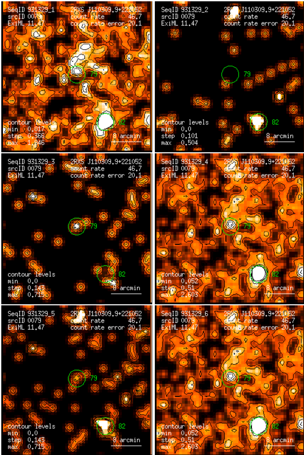
Figure 79: RASS 931329: detection 0079: band rate images, Gaussian filter: (1) PSPC channels 11 – 41, (2) 52 – 90, (3) 91 – 201, (4) 11 – 235, (5) 52 – 201, (6) 11 – 201. Broad band rates in counts/ks. Band rate contour levels in counts/ks/arcmin 2 .
