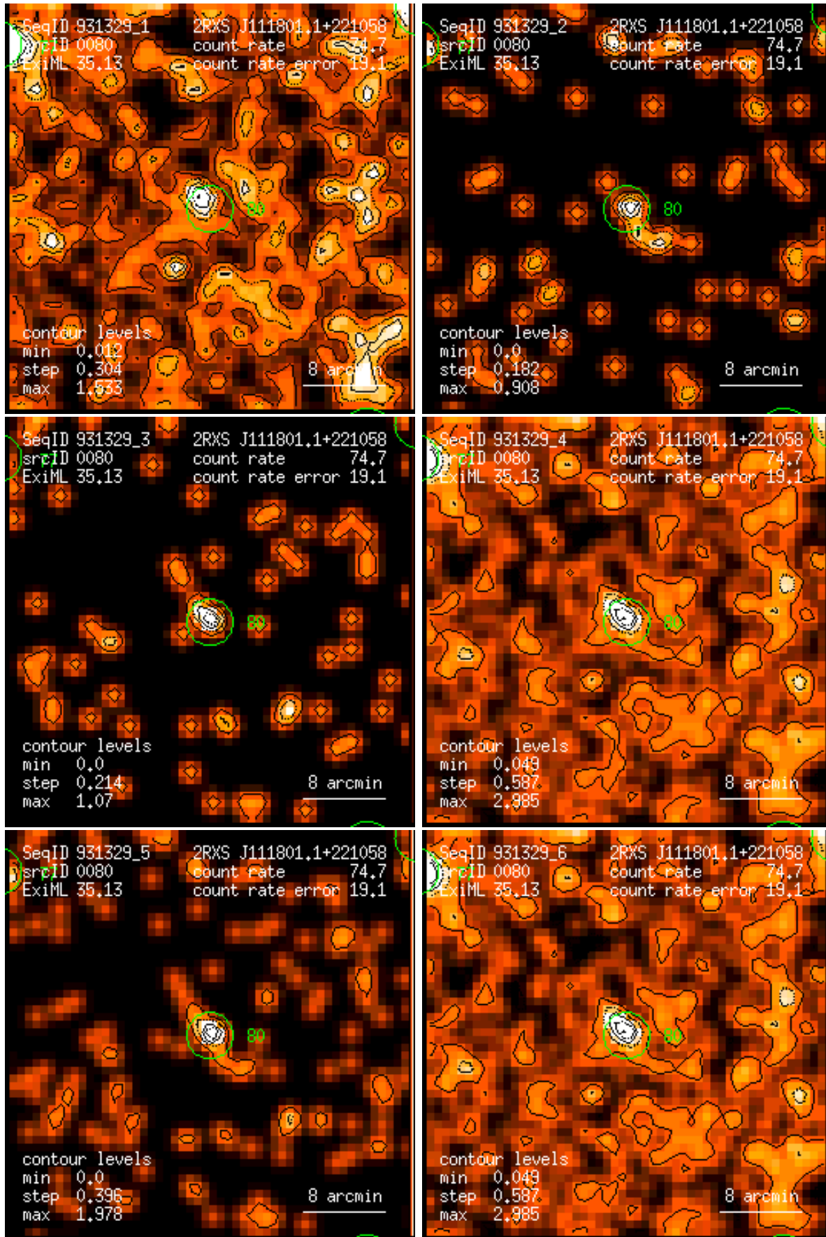
Figure 80: RASS 931329: detection 0080: band rate images, Gaussian filter: (1) PSPC channels 11 – 41, (2) 52 – 90, (3) 91 – 201, (4) 11 – 235, (5) 52 – 201, (6) 11 – 201. Broad band rates in counts/ks. Band rate contour levels in counts/ks/arcmin 2 .
