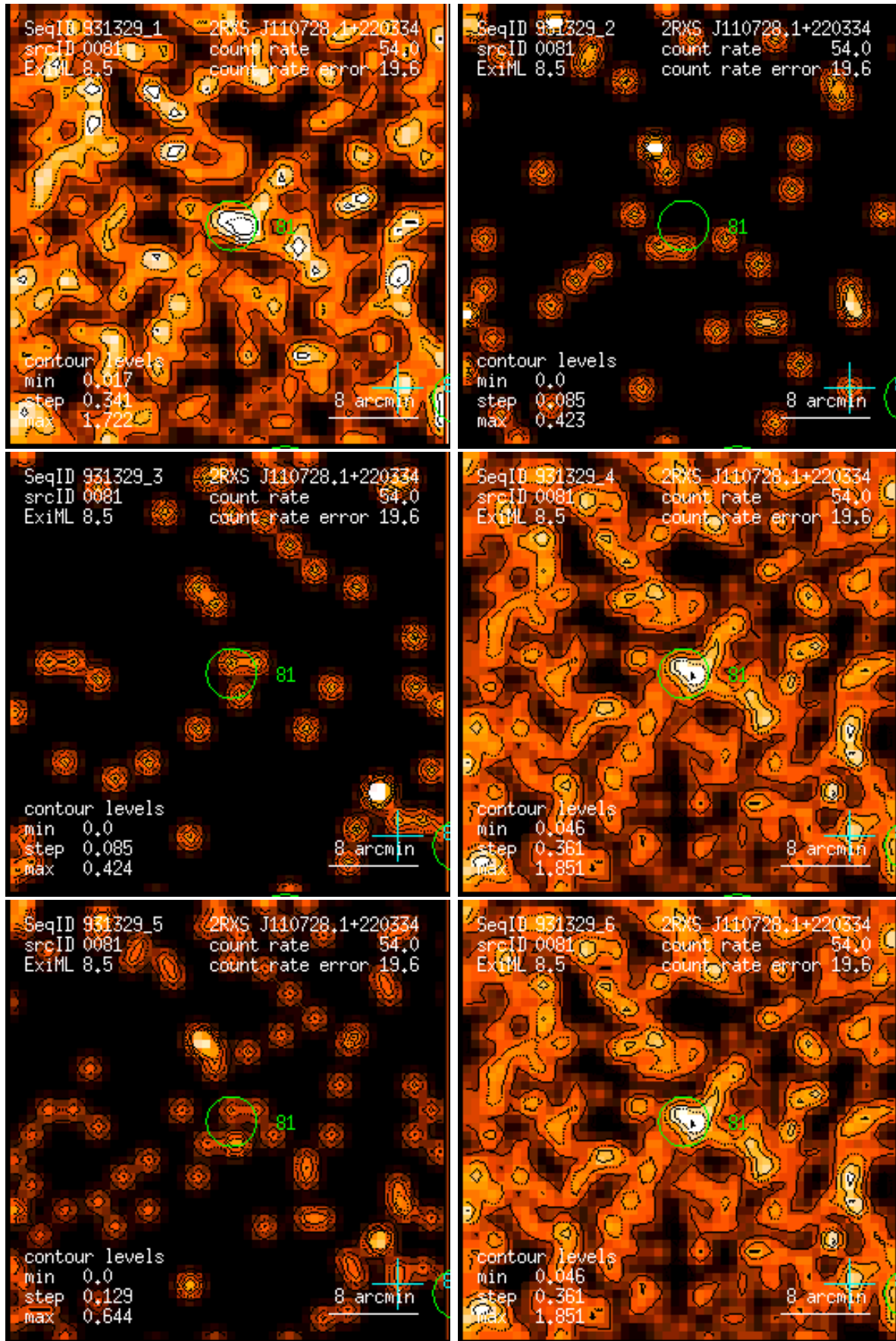
Figure 81: RASS 931329: detection 0081: band rate images, Gaussian filter: (1) PSPC channels 11 – 41, (2) 52 – 90, (3) 91 – 201, (4) 11 – 235, (5) 52 – 201, (6) 11 – 201. Broad band rates in counts/ks. Band rate contour levels in counts/ks/arcmin 2 .
