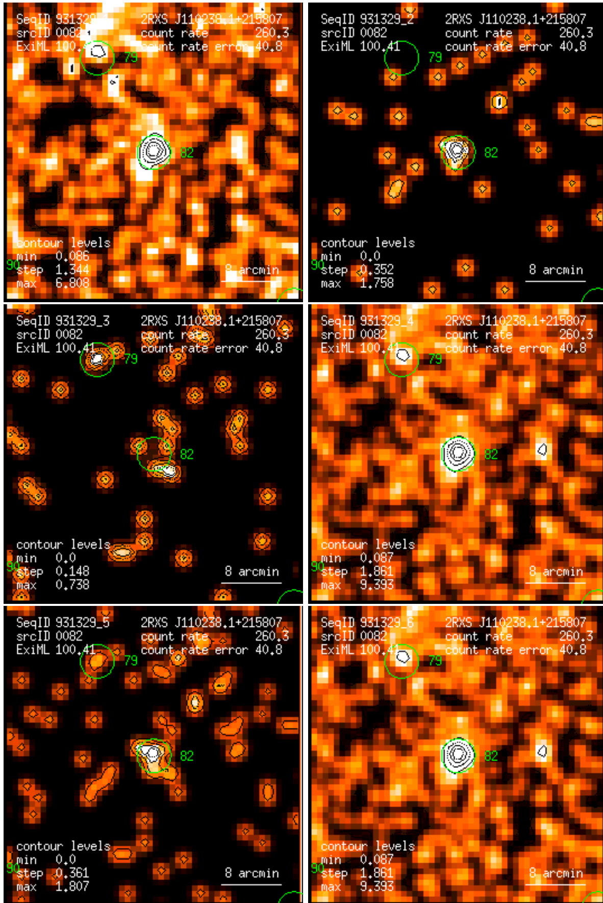
Figure 82: RASS 931329: detection 0082: band rate images, Gaussian filter: (1) PSPC channels 11 – 41, (2) 52 – 90, (3) 91 – 201, (4) 11 – 235, (5) 52 – 201, (6) 11 – 201. Broad band rates in counts/ks. Band rate contour levels in counts/ks/arcmin 2 .
