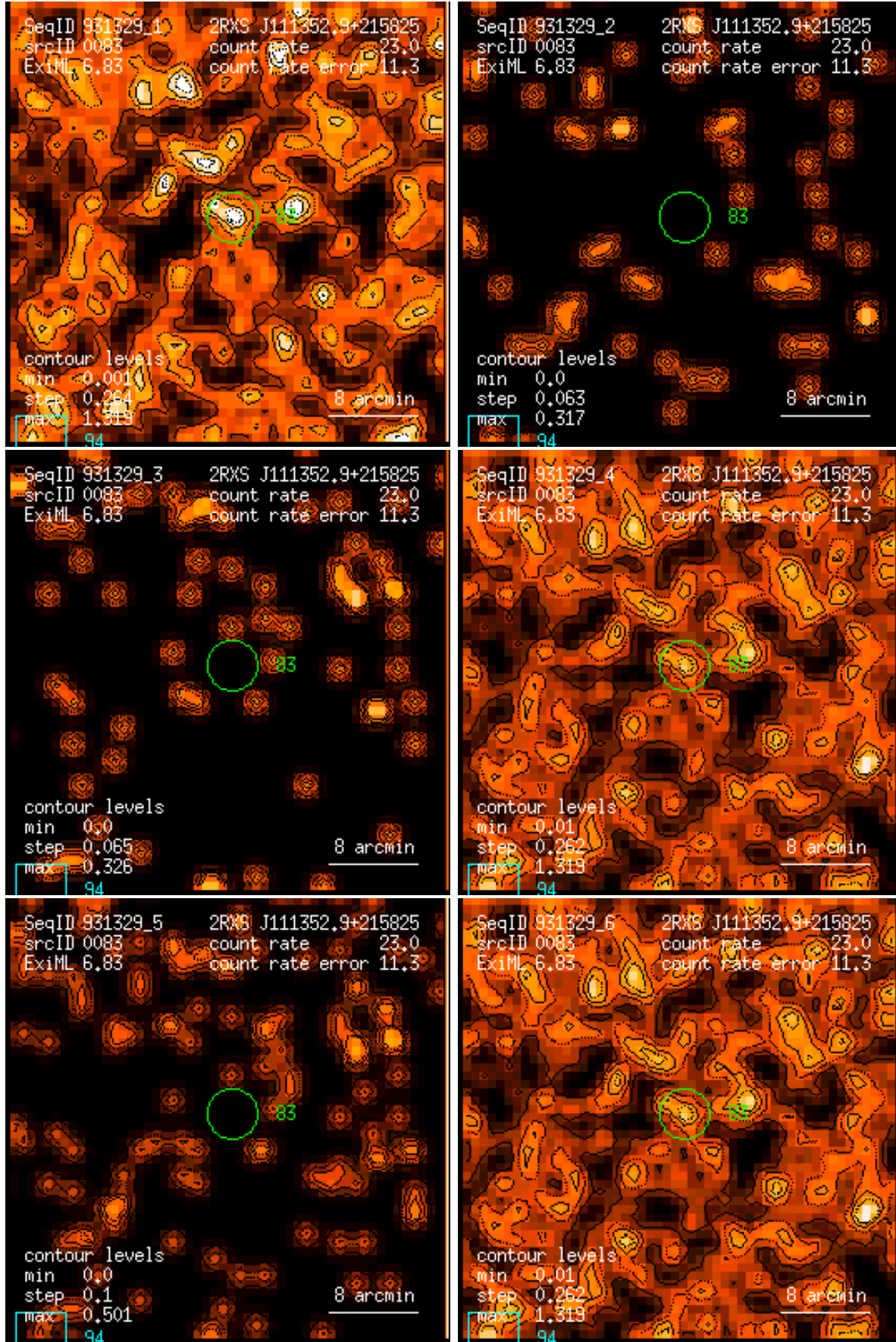
Figure 83: RASS 931329: detection 0083: band rate images, Gaussian filter: (1) PSPC channels 11 – 41, (2) 52 – 90, (3) 91 – 201, (4) 11 – 235, (5) 52 – 201, (6) 11 – 201. Broad band rates in counts/ks. Band rate contour levels in counts/ks/arcmin 2 .
