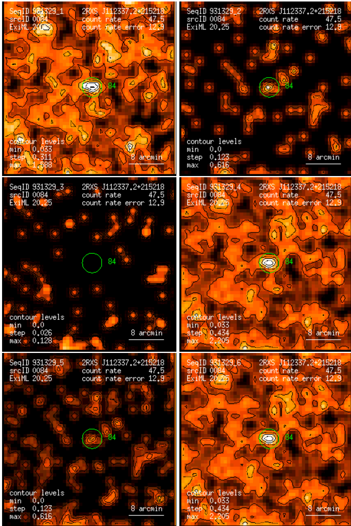
Figure 84: RASS 931329: detection 0084: band rate images, Gaussian filter: (1) PSPC channels 11 – 41, (2) 52 – 90, (3) 91 – 201, (4) 11 – 235, (5) 52 – 201, (6) 11 – 201. Broad band rates in counts/ks. Band rate contour levels in counts/ks/arcmin 2 .
