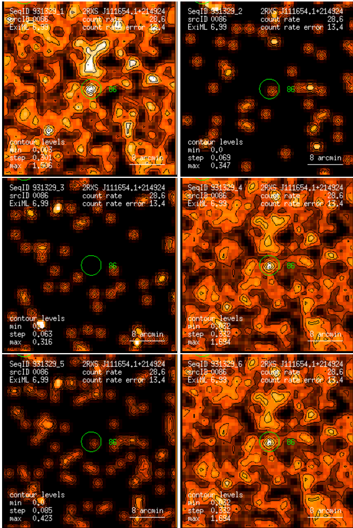
Figure 86: RASS 931329: detection 0086: band rate images, Gaussian filter: (1) PSPC channels 11 – 41, (2) 52 – 90, (3) 91 – 201, (4) 11 – 235, (5) 52 – 201, (6) 11 – 201. Broad band rates in counts/ks. Band rate contour levels in counts/ks/arcmin 2 .
