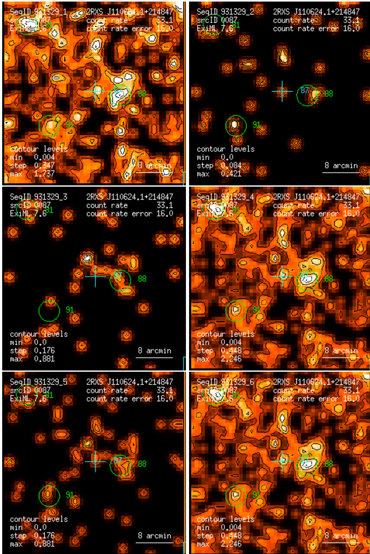
Figure 87: RASS 931329: detection 0087: band rate images, Gaussian filter: (1) PSPC channels 11 – 41, (2) 52 – 90, (3) 91 – 201, (4) 11 – 235, (5) 52 – 201, (6) 11 – 201. Broad band rates in counts/ks. Band rate contour levels in counts/ks/arcmin 2 .
