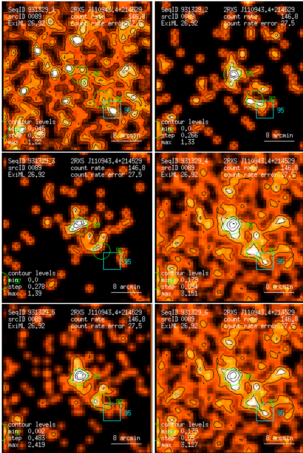
Figure 89: RASS 931329: detection 0089: band rate images, Gaussian filter: (1) PSPC channels 11 – 41, (2) 52 – 90, (3) 91 – 201, (4) 11 – 235, (5) 52 – 201, (6) 11 – 201. Broad band rates in counts/ks. Band rate contour levels in counts/ks/arcmin 2 .
