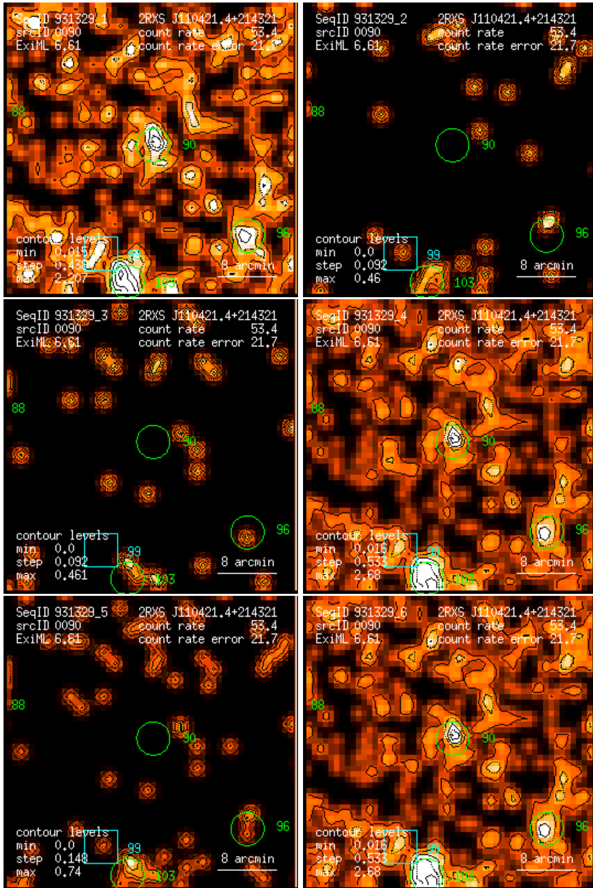
Figure 90: RASS 931329: detection 0090: band rate images, Gaussian filter: (1) PSPC channels 11 – 41, (2) 52 – 90, (3) 91 – 201, (4) 11 – 235, (5) 52 – 201, (6) 11 – 201. Broad band rates in counts/ks. Band rate contour levels in counts/ks/arcmin 2 .
