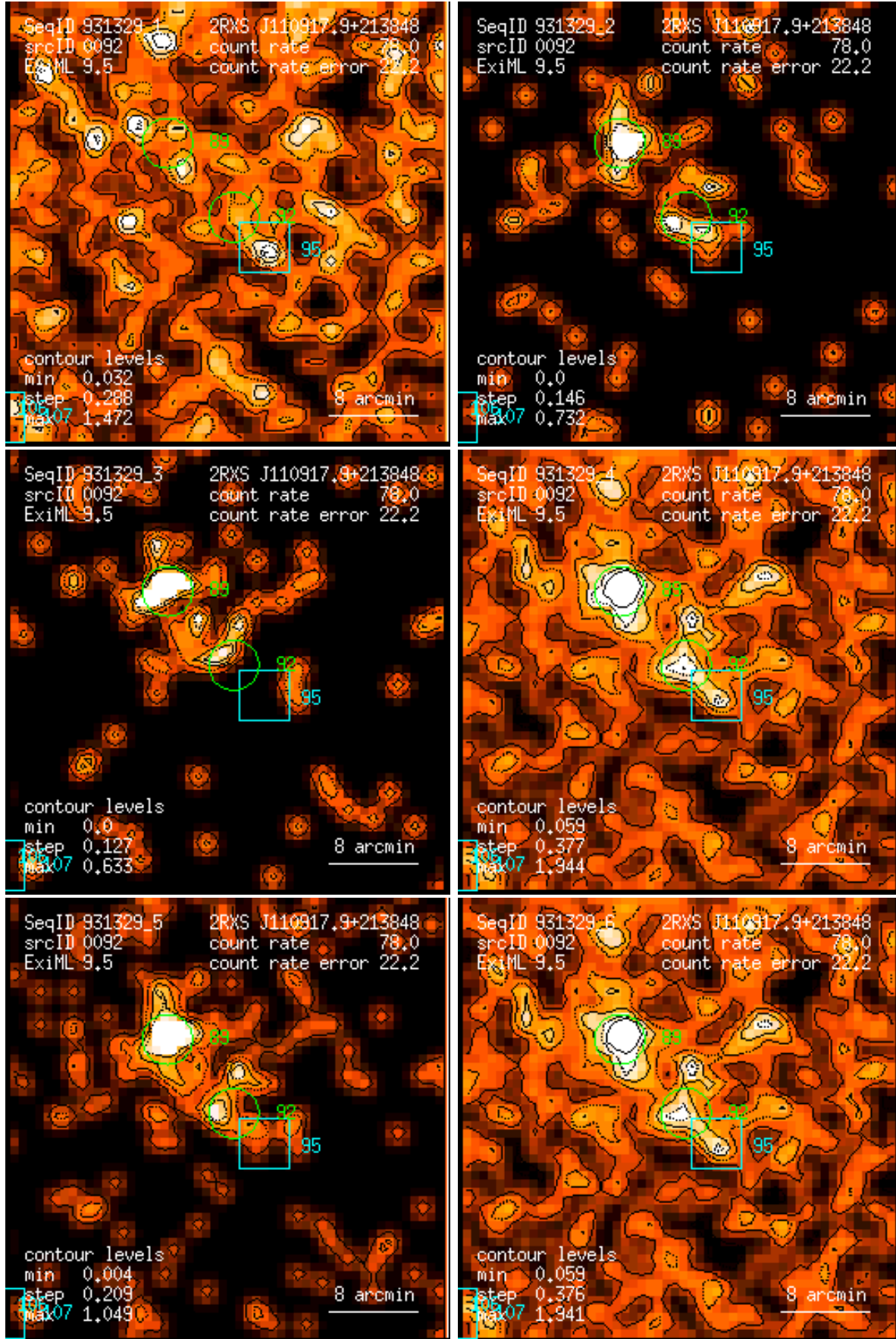
Figure 92: RASS 931329: detection 0092: band rate images, Gaussian filter: (1) PSPC channels 11 – 41, (2) 52 – 90, (3) 91 – 201, (4) 11 – 235, (5) 52 – 201, (6) 11 – 201. Broad band rates in counts/ks. Band rate contour levels in counts/ks/arcmin 2 .
