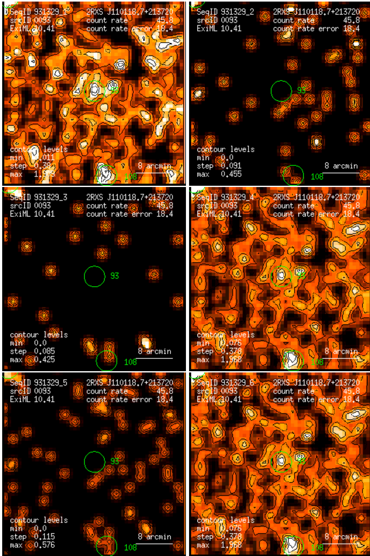
Figure 93: RASS 931329: detection 0093: band rate images, Gaussian filter: (1) PSPC channels 11 – 41, (2) 52 – 90, (3) 91 – 201, (4) 11 – 235, (5) 52 – 201, (6) 11 – 201. Broad band rates in counts/ks. Band rate contour levels in counts/ks/arcmin 2 .
