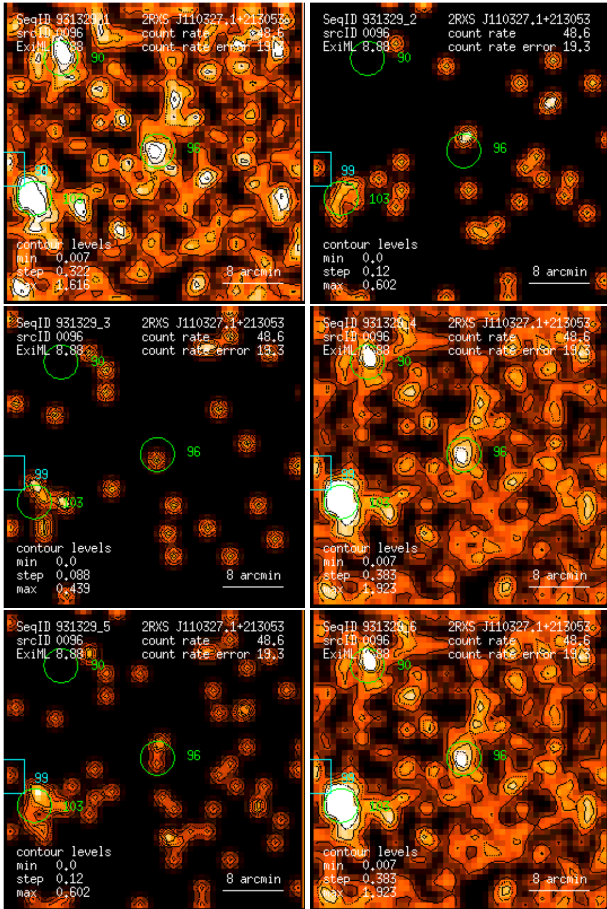
Figure 96: RASS 931329: detection 0096: band rate images, Gaussian filter: (1) PSPC channels 11 – 41, (2) 52 – 90, (3) 91 – 201, (4) 11 – 235, (5) 52 – 201, (6) 11 – 201. Broad band rates in counts/ks. Band rate contour levels in counts/ks/arcmin 2 .
