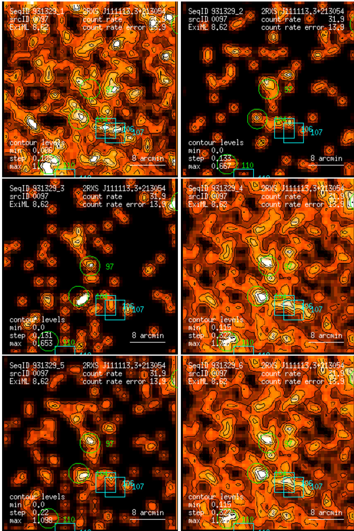
Figure 97: RASS 931329: detection 0097: band rate images, Gaussian filter: (1) PSPC channels 11 – 41, (2) 52 – 90, (3) 91 – 201, (4) 11 – 235, (5) 52 – 201, (6) 11 – 201. Broad band rates in counts/ks. Band rate contour levels in counts/ks/arcmin 2 .
