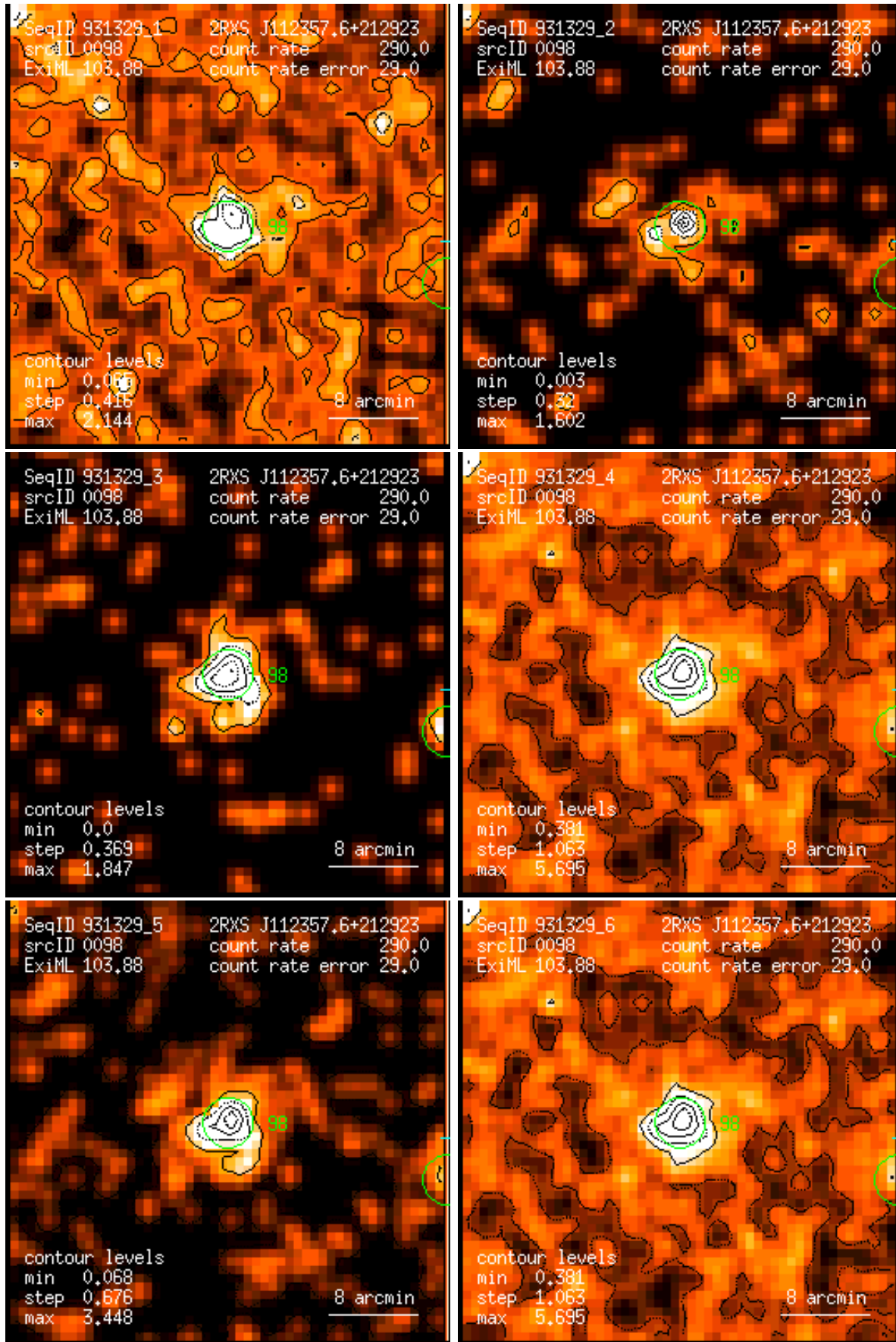
Figure 98: RASS 931329: detection 0098: band rate images, Gaussian filter: (1) PSPC channels 11 – 41, (2) 52 – 90, (3) 91 – 201, (4) 11 – 235, (5) 52 – 201, (6) 11 – 201. Broad band rates in counts/ks. Band rate contour levels in counts/ks/arcmin 2 .
