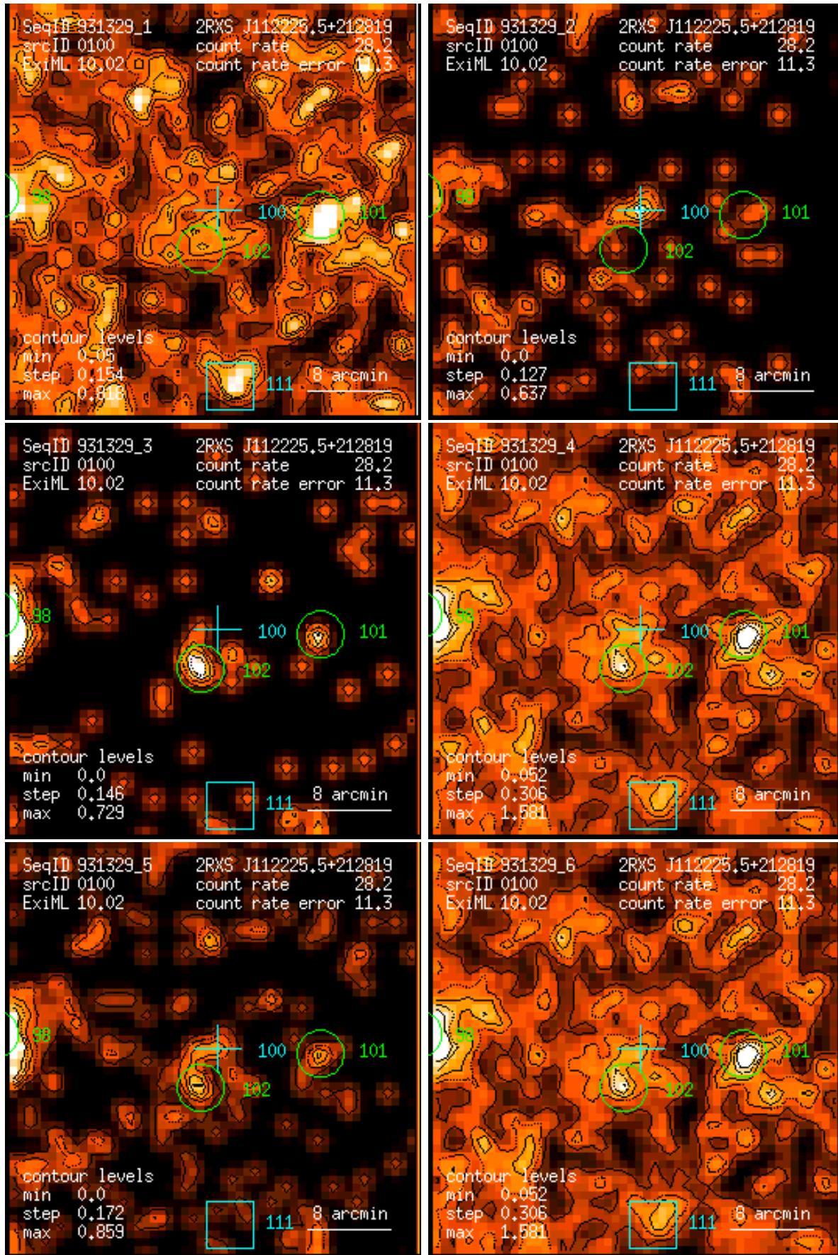
Figure 100: RASS 931329: detection 0100: band rate images, Gaussian filter: (1) PSPC channels 11 – 41, (2) 52 – 90, (3) 91 – 201, (4) 11 – 235, (5) 52 – 201, (6) 11 – 201. Broad band rates in counts/ks. Band rate contour levels in counts/ks/arcmin 2 .
