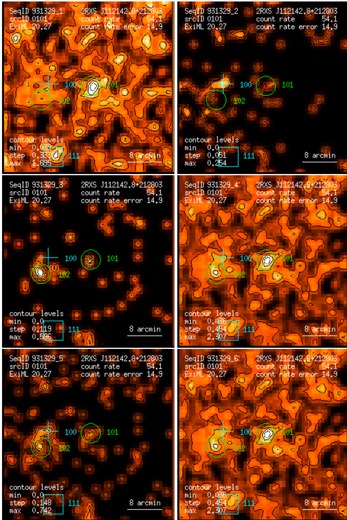
Figure 101: RASS 931329: detection 0101: band rate images, Gaussian filter: (1) PSPC channels 11 – 41, (2) 52 – 90, (3) 91 – 201, (4) 11 – 235, (5) 52 – 201, (6) 11 – 201. Broad band rates in counts/ks. Band rate contour levels in counts/ks/arcmin 2 .
