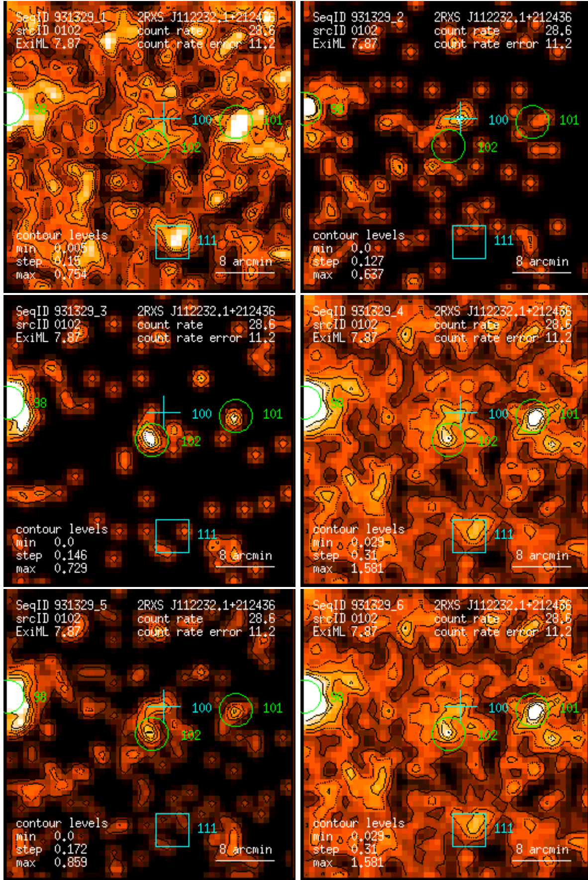
Figure 102: RASS 931329: detection 0102: band rate images, Gaussian filter: (1) PSPC channels 11 – 41, (2) 52 – 90, (3) 91 – 201, (4) 11 – 235, (5) 52 – 201, (6) 11 – 201. Broad band rates in counts/ks. Band rate contour levels in counts/ks/arcmin 2 .
