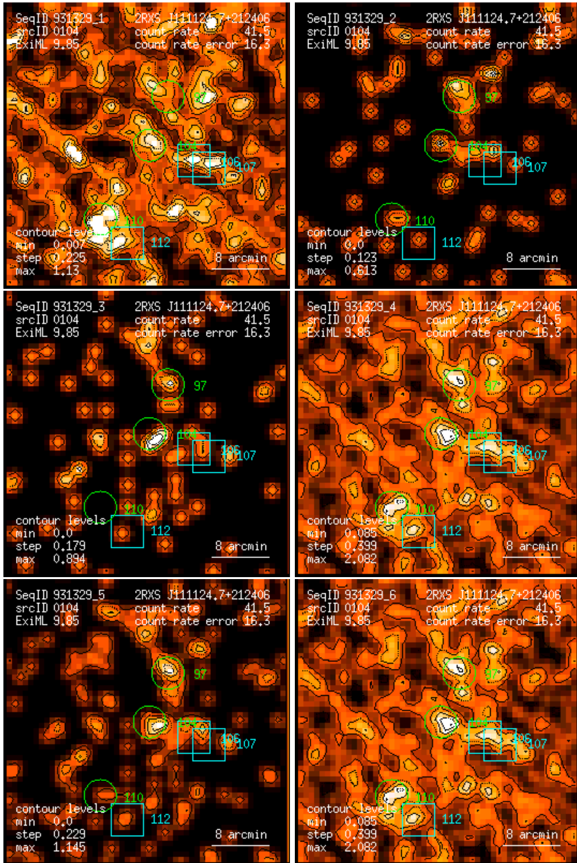
Figure 104: RASS 931329: detection 0104: band rate images, Gaussian filter: (1) PSPC channels 11 – 41, (2) 52 – 90, (3) 91 – 201, (4) 11 – 235, (5) 52 – 201, (6) 11 – 201. Broad band rates in counts/ks. Band rate contour levels in counts/ks/arcmin 2 .
