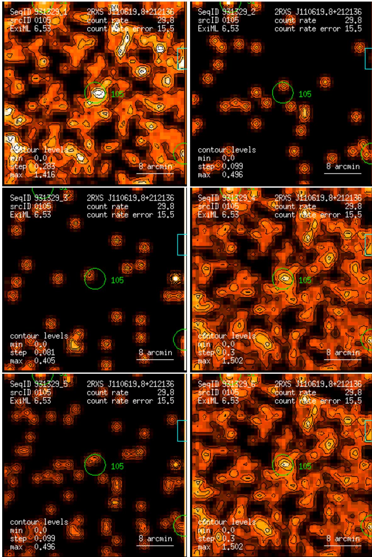
Figure 105: RASS 931329: detection 0105: band rate images, Gaussian filter: (1) PSPC channels 11 – 41, (2) 52 – 90, (3) 91 – 201, (4) 11 – 235, (5) 52 – 201, (6) 11 – 201. Broad band rates in counts/ks. Band rate contour levels in counts/ks/arcmin 2 .
