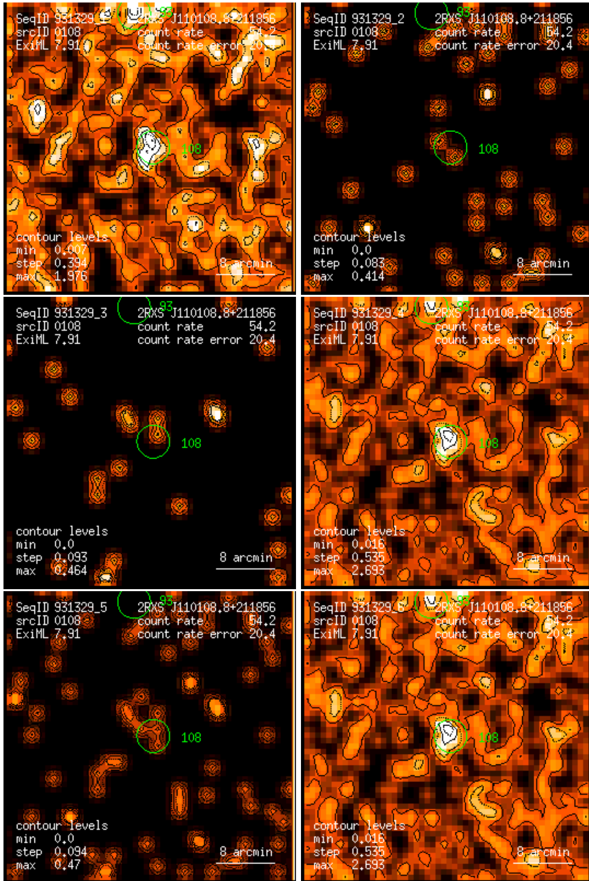
Figure 108: RASS 931329: detection 0108: band rate images, Gaussian filter: (1) PSPC channels 11 – 41, (2) 52 – 90, (3) 91 – 201, (4) 11 – 235, (5) 52 – 201, (6) 11 – 201. Broad band rates in counts/ks. Band rate contour levels in counts/ks/arcmin 2 .
