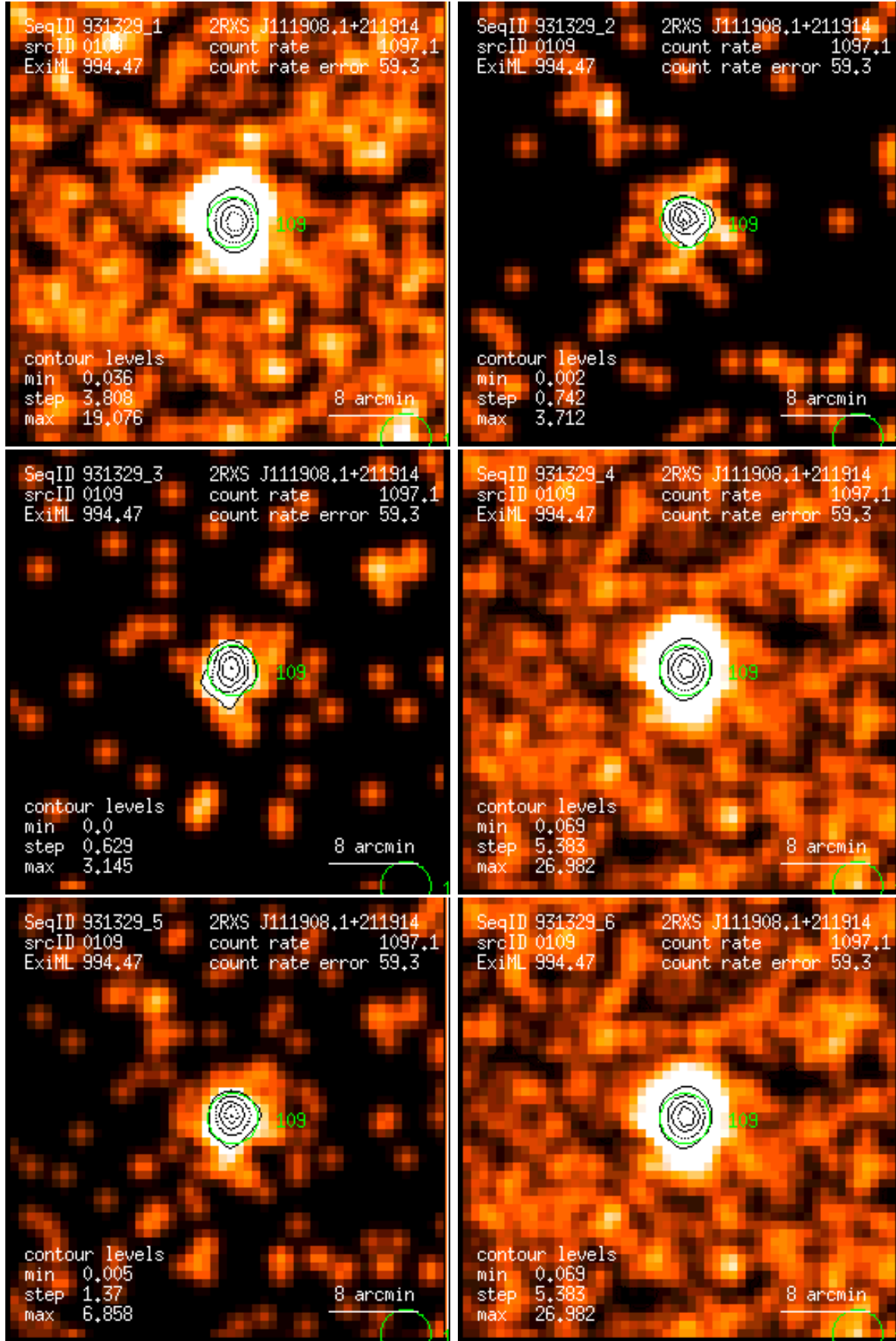
Figure 109: RASS 931329: detection 0109: band rate images, Gaussian filter: (1) PSPC channels 11 – 41, (2) 52 – 90, (3) 91 – 201, (4) 11 – 235, (5) 52 – 201, (6) 11 – 201. Broad band rates in counts/ks. Band rate contour levels in counts/ks/arcmin 2 .
