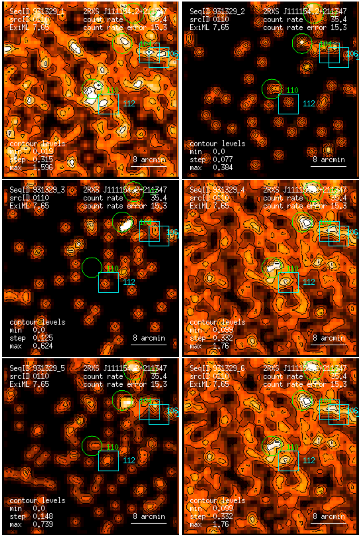
Figure 110: RASS 931329: detection 0110: band rate images, Gaussian filter: (1) PSPC channels 11 – 41, (2) 52 – 90, (3) 91 – 201, (4) 11 – 235, (5) 52 – 201, (6) 11 – 201. Broad band rates in counts/ks. Band rate contour levels in counts/ks/arcmin 2 .
