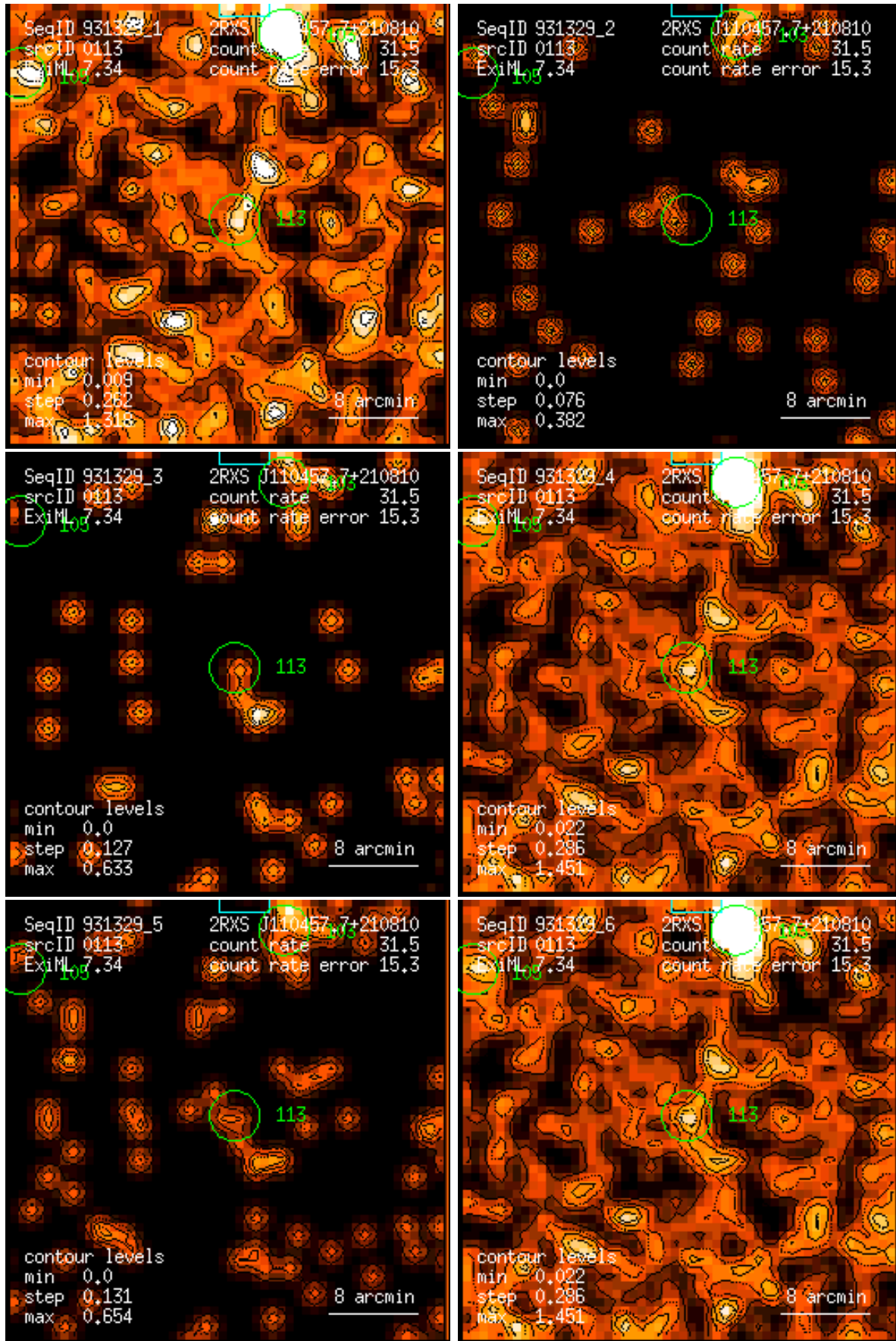
Figure 113: RASS 931329: detection 0113: band rate images, Gaussian filter: (1) PSPC channels 11 – 41, (2) 52 – 90, (3) 91 – 201, (4) 11 – 235, (5) 52 – 201, (6) 11 – 201. Broad band rates in counts/ks. Band rate contour levels in counts/ks/arcmin 2 .
