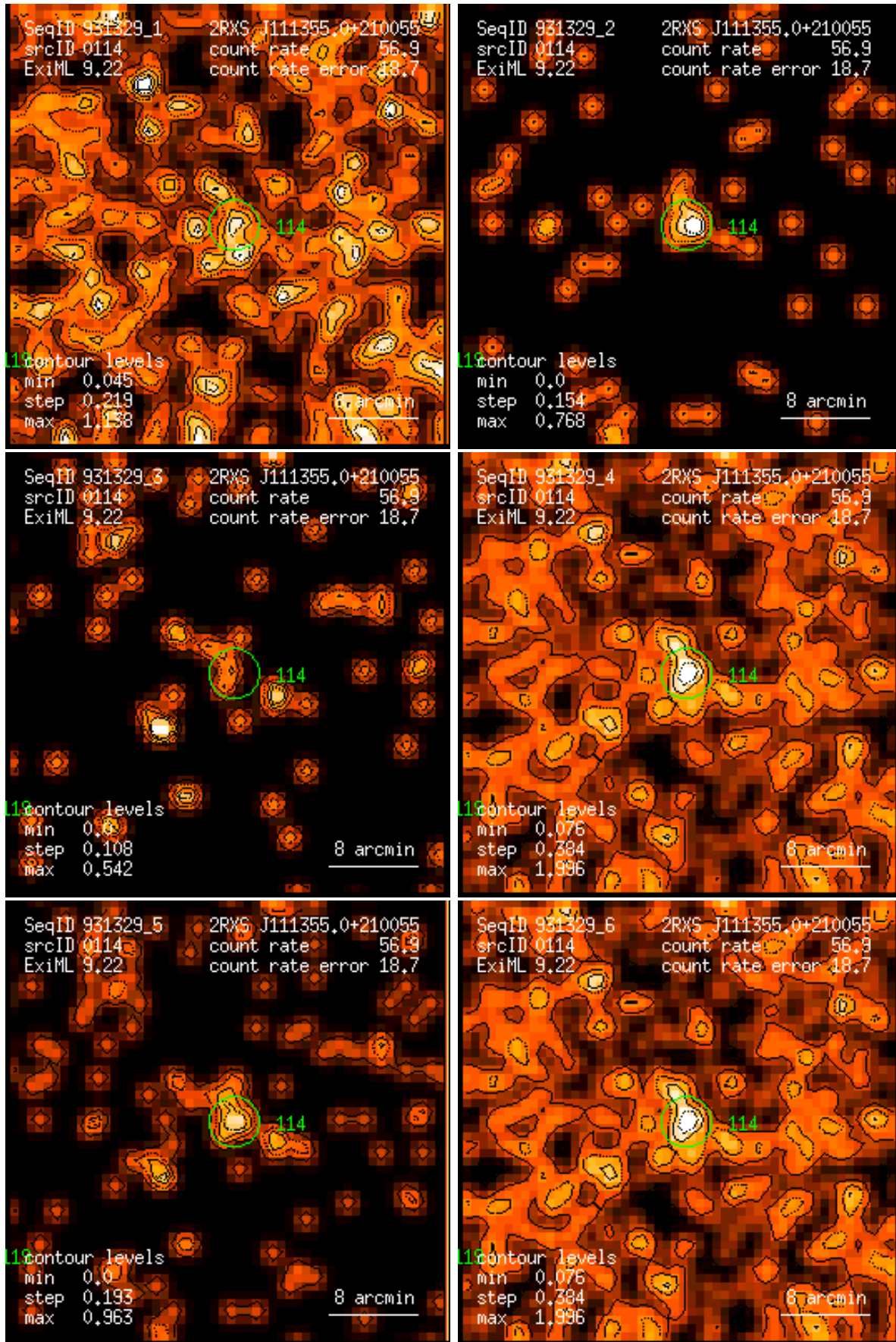
Figure 114: RASS 931329: detection 0114: band rate images, Gaussian filter: (1) PSPC channels 11 – 41, (2) 52 – 90, (3) 91 – 201, (4) 11 – 235, (5) 52 – 201, (6) 11 – 201. Broad band rates in counts/ks. Band rate contour levels in counts/ks/arcmin 2 .
