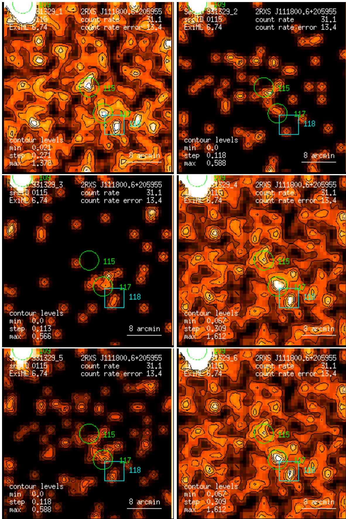
Figure 115: RASS 931329: detection 0115: band rate images, Gaussian filter: (1) PSPC channels 11 – 41, (2) 52 – 90, (3) 91 – 201, (4) 11 – 235, (5) 52 – 201, (6) 11 – 201. Broad band rates in counts/ks. Band rate contour levels in counts/ks/arcmin 2 .
