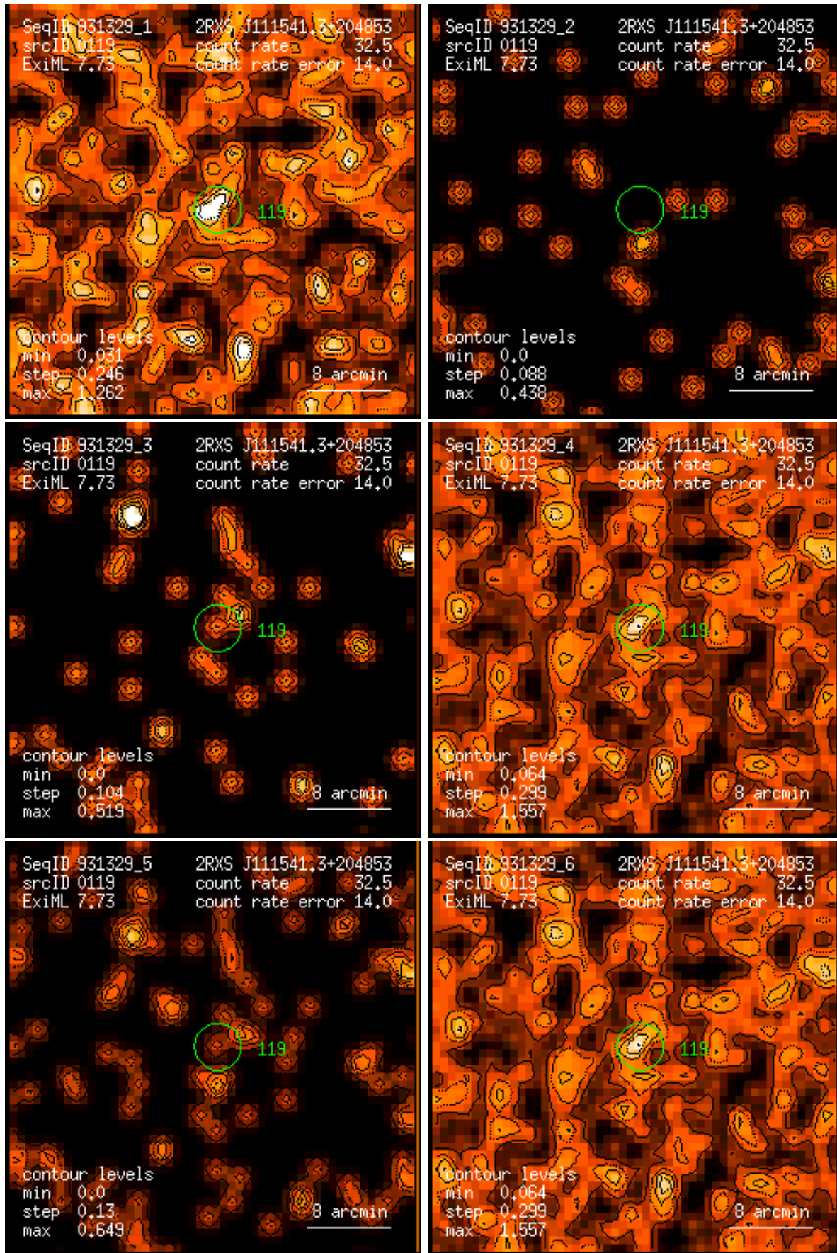
Figure 119: RASS 931329: detection 0119: band rate images, Gaussian filter: (1) PSPC channels 11 – 41, (2) 52 – 90, (3) 91 – 201, (4) 11 – 235, (5) 52 – 201, (6) 11 – 201. Broad band rates in counts/ks. Band rate contour levels in counts/ks/arcmin 2 .
