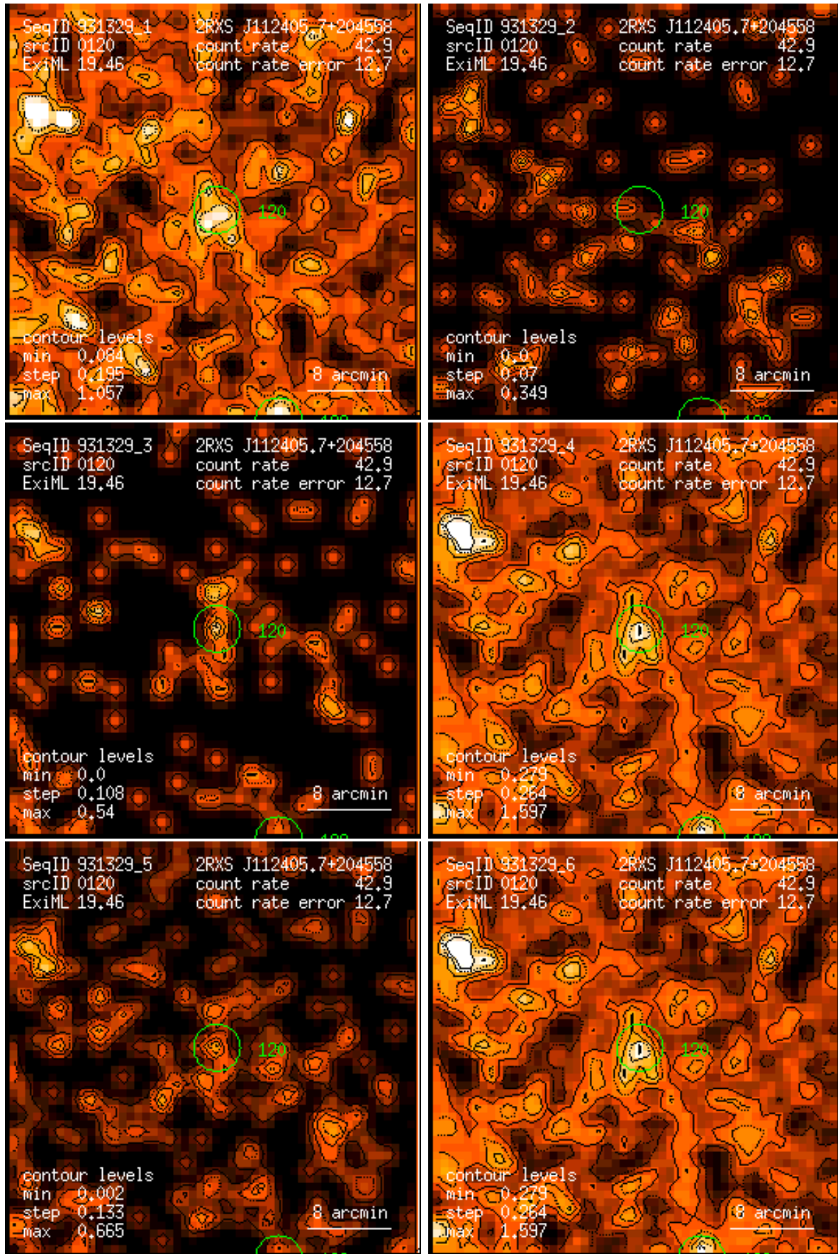
Figure 120: RASS 931329: detection 0120: band rate images, Gaussian filter: (1) PSPC channels 11 – 41, (2) 52 – 90, (3) 91 – 201, (4) 11 – 235, (5) 52 – 201, (6) 11 – 201. Broad band rates in counts/ks. Band rate contour levels in counts/ks/arcmin 2 .
