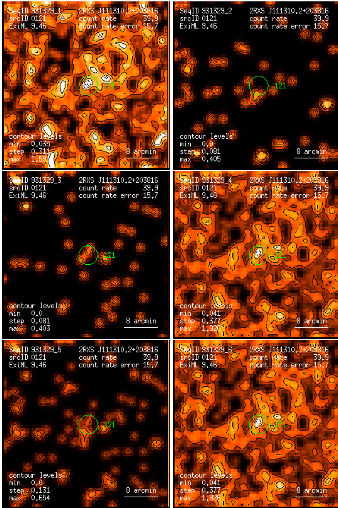
Figure 121: RASS 931329: detection 0121: band rate images, Gaussian filter: (1) PSPC channels 11 – 41, (2) 52 – 90, (3) 91 – 201, (4) 11 – 235, (5) 52 – 201, (6) 11 – 201. Broad band rates in counts/ks. Band rate contour levels in counts/ks/arcmin 2 .
