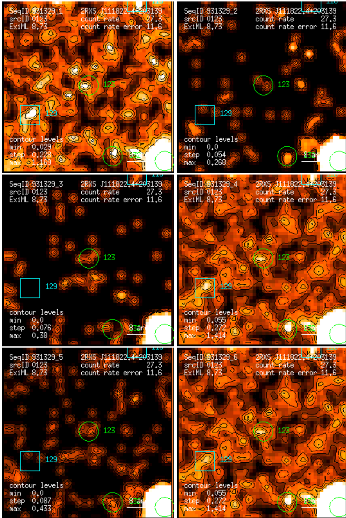
Figure 123: RASS 931329: detection 0123: band rate images, Gaussian filter: (1) PSPC channels 11 – 41, (2) 52 – 90, (3) 91 – 201, (4) 11 – 235, (5) 52 – 201, (6) 11 – 201. Broad band rates in counts/ks. Band rate contour levels in counts/ks/arcmin 2 .
