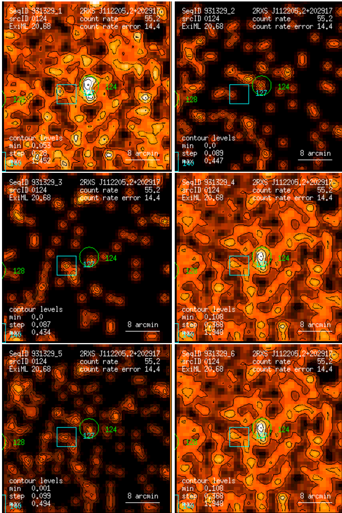
Figure 124: RASS 931329: detection 0124: band rate images, Gaussian filter: (1) PSPC channels 11 – 41, (2) 52 – 90, (3) 91 – 201, (4) 11 – 235, (5) 52 – 201, (6) 11 – 201. Broad band rates in counts/ks. Band rate contour levels in counts/ks/arcmin 2 .
