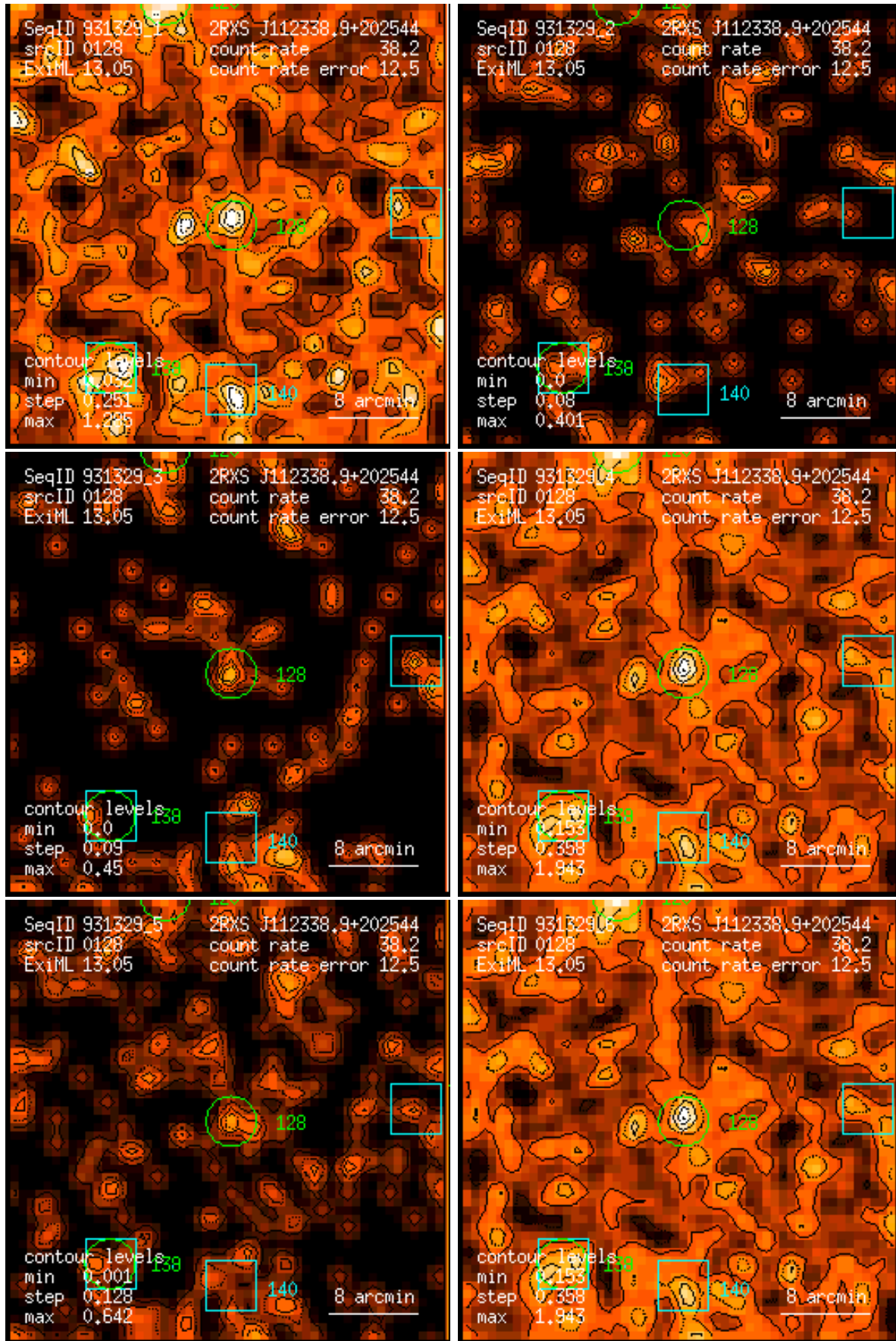
Figure 128: RASS 931329: detection 0128: band rate images, Gaussian filter: (1) PSPC channels 11 – 41, (2) 52 – 90, (3) 91 – 201, (4) 11 – 235, (5) 52 – 201, (6) 11 – 201. Broad band rates in counts/ks. Band rate contour levels in counts/ks/arcmin 2 .
