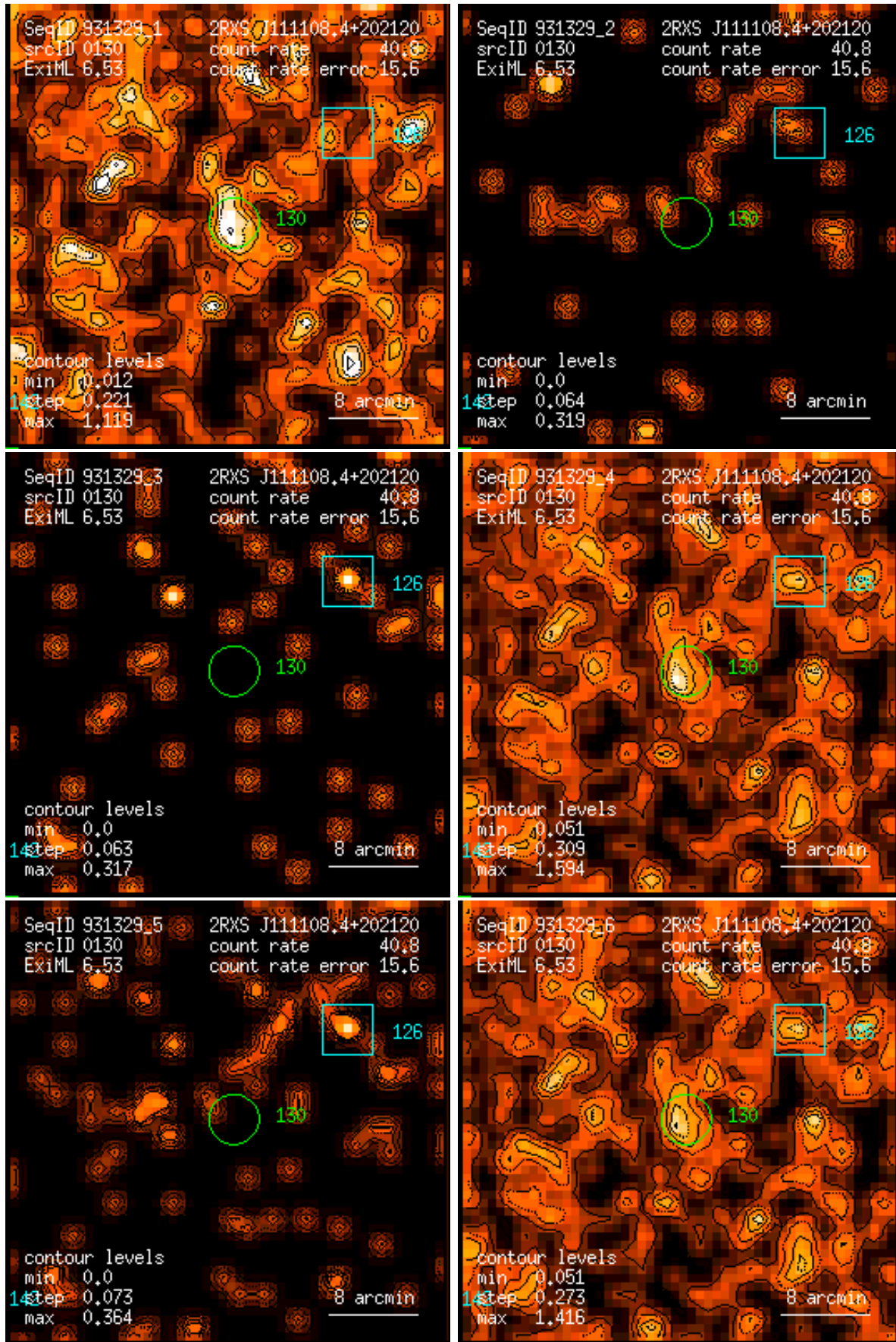
Figure 130: RASS 931329: detection 0130: band rate images, Gaussian filter: (1) PSPC channels 11 – 41, (2) 52 – 90, (3) 91 – 201, (4) 11 – 235, (5) 52 – 201, (6) 11 – 201. Broad band rates in counts/ks. Band rate contour levels in counts/ks/arcmin 2 .
