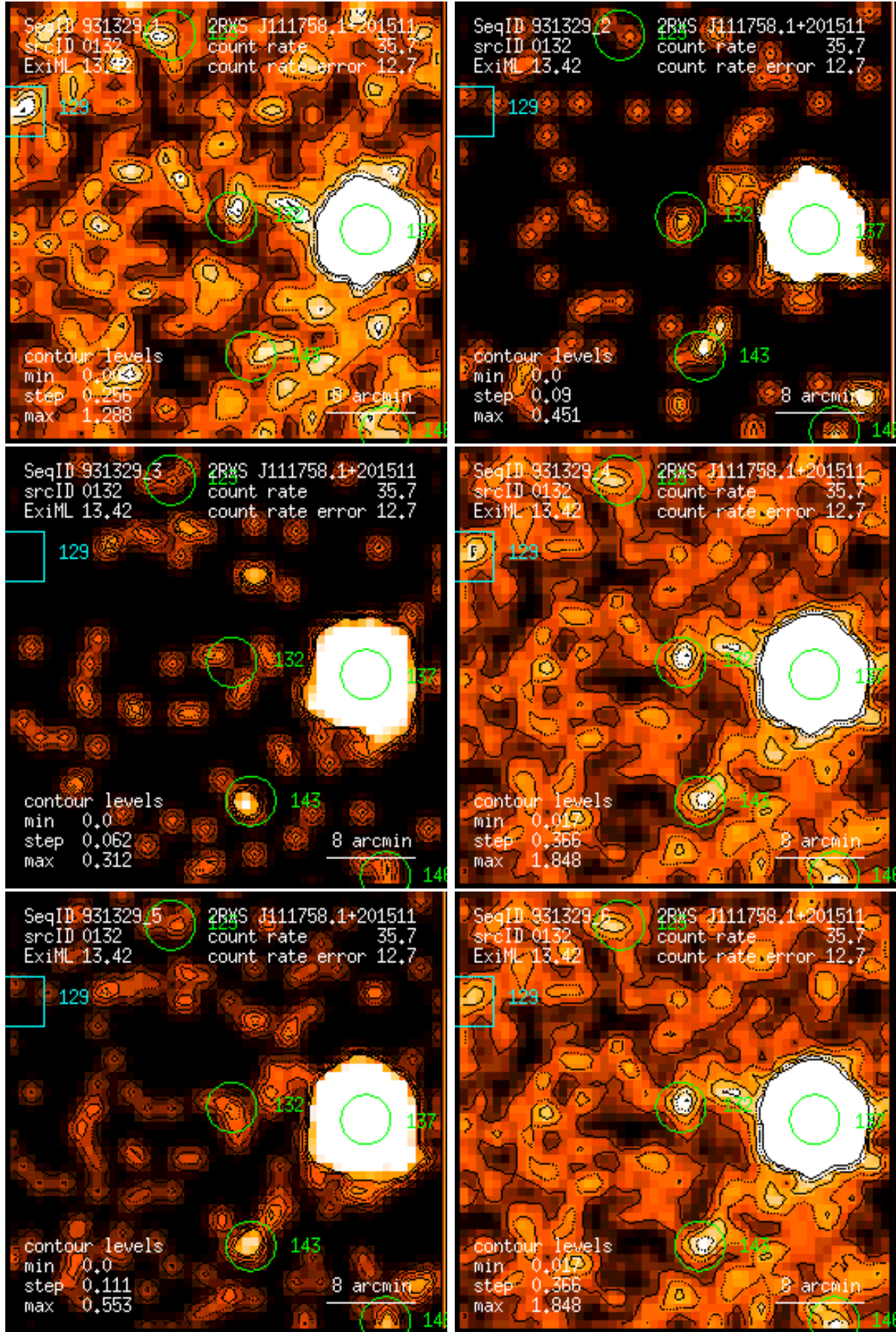
Figure 132: RASS 931329: detection 0132: band rate images, Gaussian filter: (1) PSPC channels 11 – 41, (2) 52 – 90, (3) 91 – 201, (4) 11 – 235, (5) 52 – 201, (6) 11 – 201. Broad band rates in counts/ks. Band rate contour levels in counts/ks/arcmin 2 .
