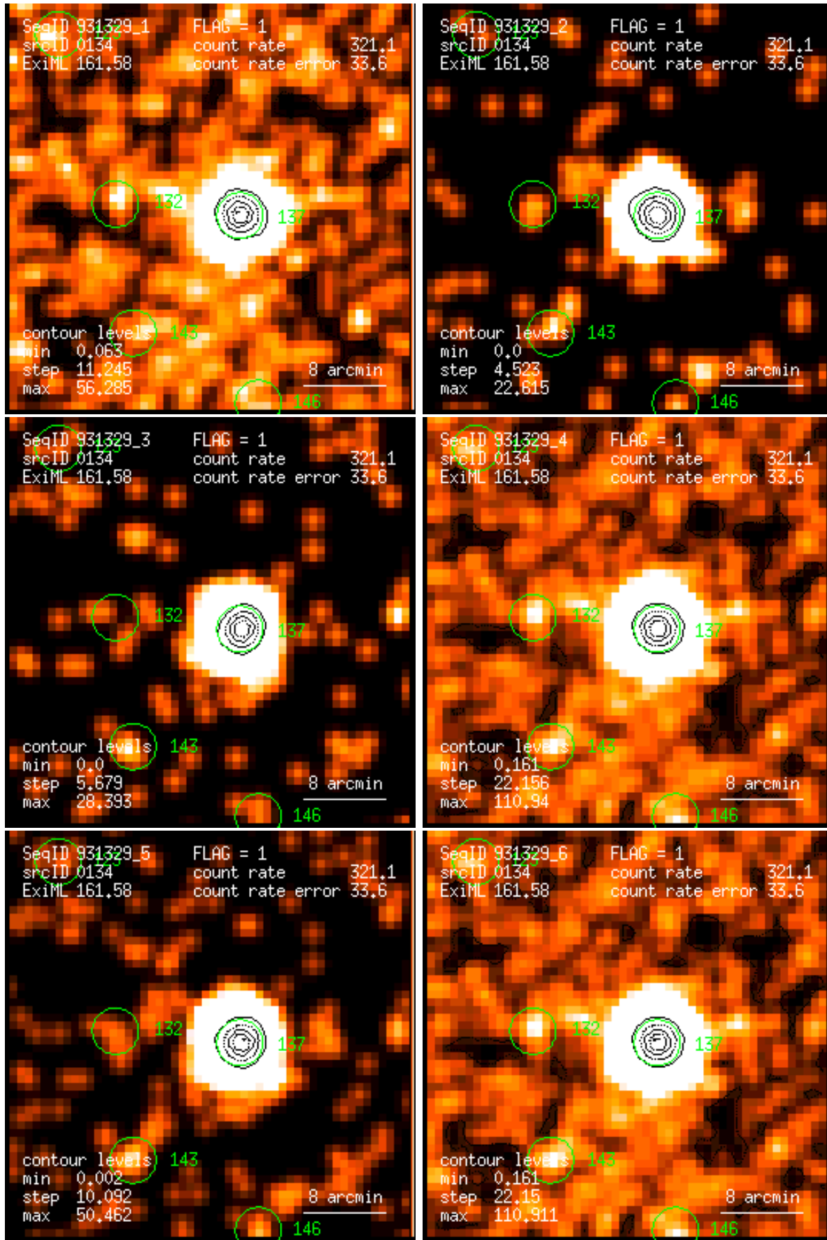
Figure 134: RASS 931329: detection 0134: band rate images, Gaussian filter: (1) PSPC channels 11 – 41, (2) 52 – 90, (3) 91 – 201, (4) 11 – 235, (5) 52 – 201, (6) 11 – 201. Broad band rates in counts/ks. Band rate contour levels in counts/ks/arcmin 2 .
