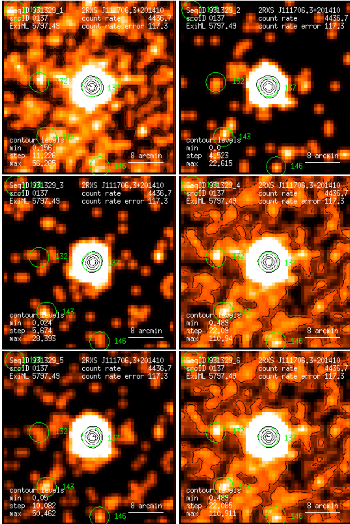
Figure 137: RASS 931329: detection 0137: band rate images, Gaussian filter: (1) PSPC channels 11 – 41, (2) 52 – 90, (3) 91 – 201, (4) 11 – 235, (5) 52 – 201, (6) 11 – 201. Broad band rates in counts/ks. Band rate contour levels in counts/ks/arcmin 2 .
