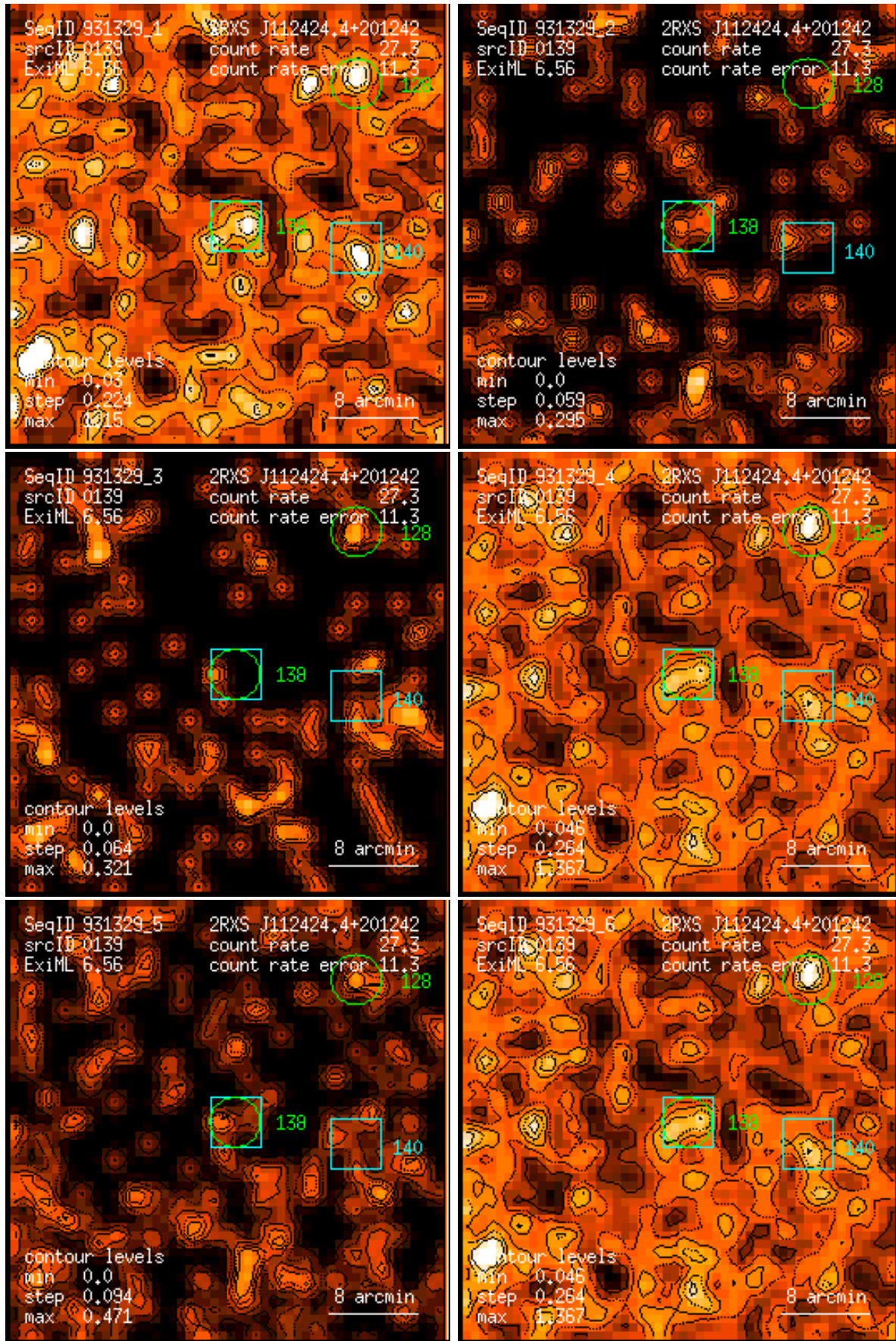
Figure 139: RASS 931329: detection 0139: band rate images, Gaussian filter: (1) PSPC channels 11 – 41, (2) 52 – 90, (3) 91 – 201, (4) 11 – 235, (5) 52 – 201, (6) 11 – 201. Broad band rates in counts/ks. Band rate contour levels in counts/ks/arcmin 2 .
