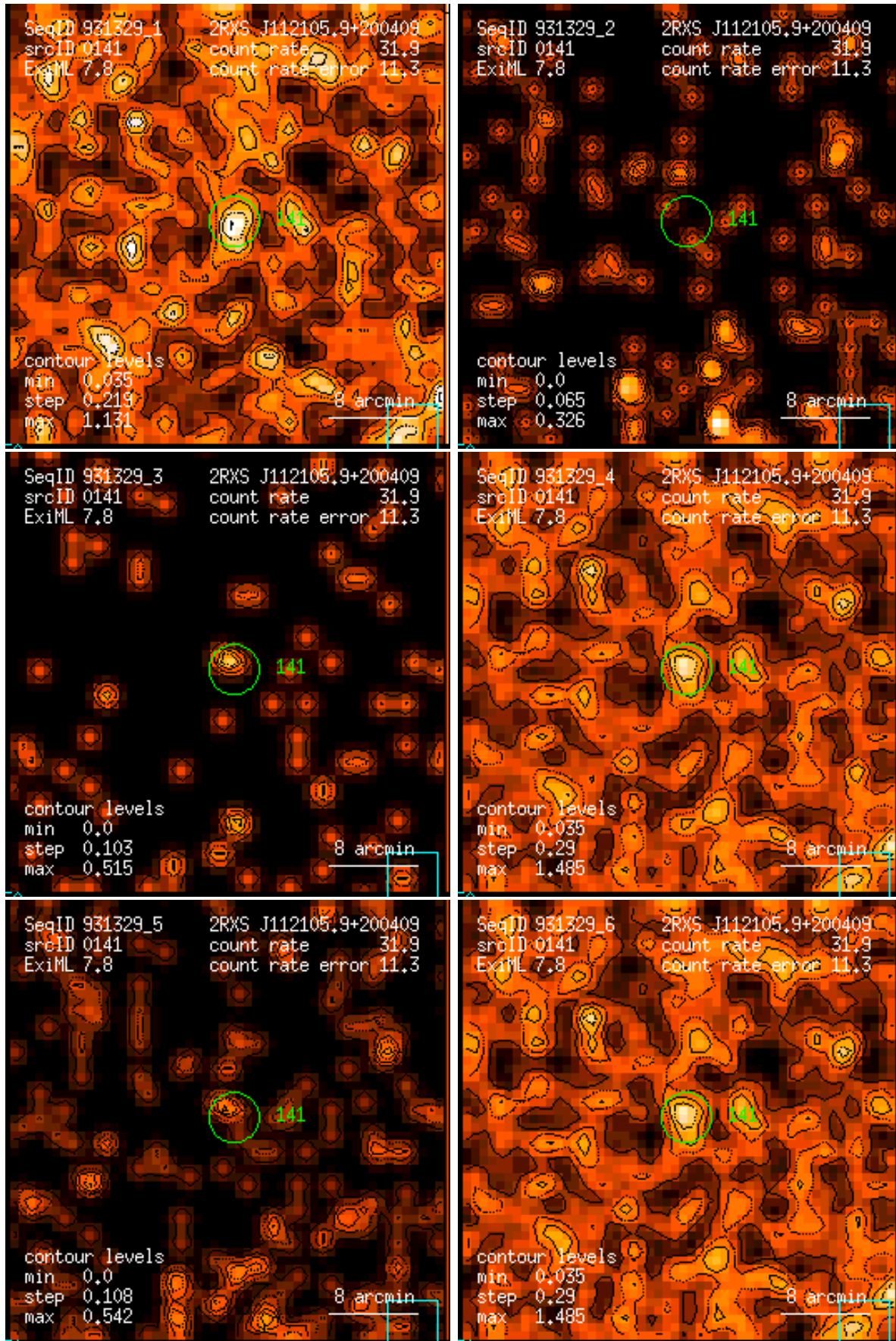
Figure 141: RASS 931329: detection 0141: band rate images, Gaussian filter: (1) PSPC channels 11 – 41, (2) 52 – 90, (3) 91 – 201, (4) 11 – 235, (5) 52 – 201, (6) 11 – 201. Broad band rates in counts/ks. Band rate contour levels in counts/ks/arcmin 2 .
