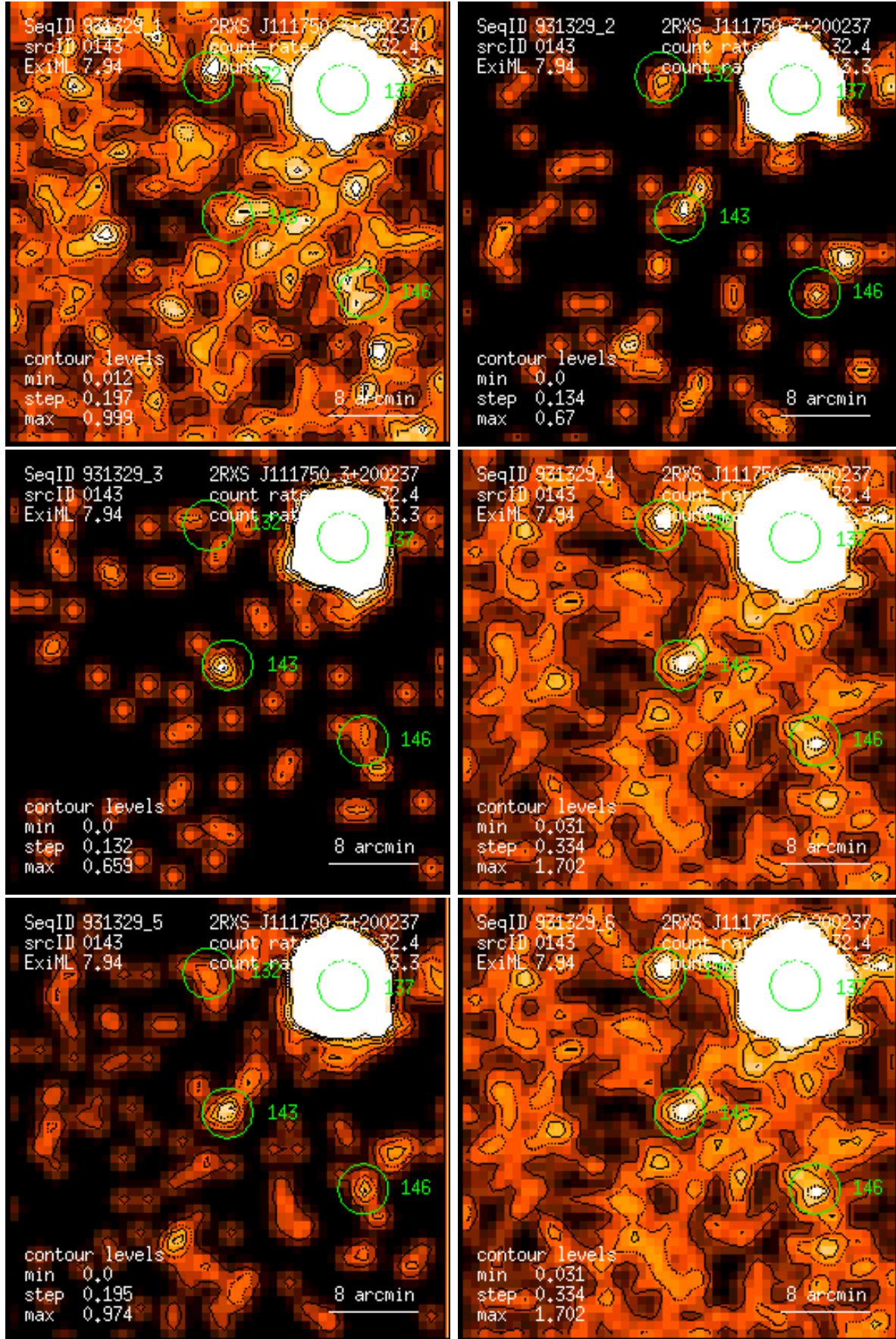
Figure 143: RASS 931329: detection 0143: band rate images, Gaussian filter: (1) PSPC channels 11 – 41, (2) 52 – 90, (3) 91 – 201, (4) 11 – 235, (5) 52 – 201, (6) 11 – 201. Broad band rates in counts/ks. Band rate contour levels in counts/ks/arcmin 2 .
