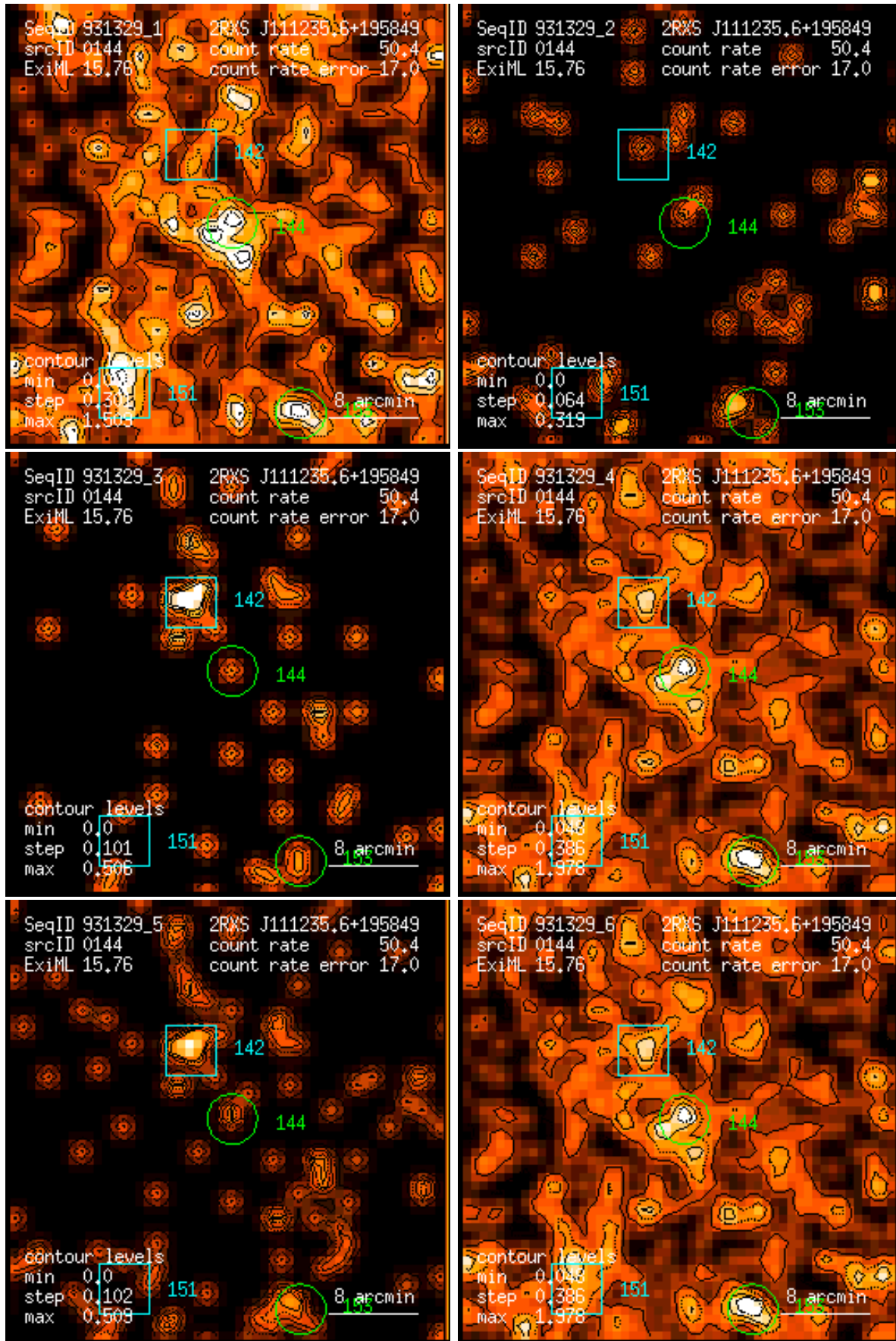
Figure 144: RASS 931329: detection 0144: band rate images, Gaussian filter: (1) PSPC channels 11 – 41, (2) 52 – 90, (3) 91 – 201, (4) 11 – 235, (5) 52 – 201, (6) 11 – 201. Broad band rates in counts/ks. Band rate contour levels in counts/ks/arcmin 2 .
