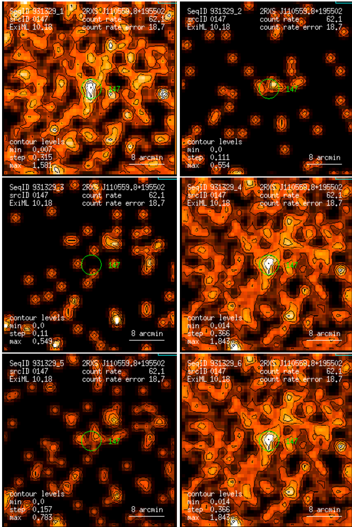
Figure 147: RASS 931329: detection 0147: band rate images, Gaussian filter: (1) PSPC channels 11 – 41, (2) 52 – 90, (3) 91 – 201, (4) 11 – 235, (5) 52 – 201, (6) 11 – 201. Broad band rates in counts/ks. Band rate contour levels in counts/ks/arcmin 2 .
