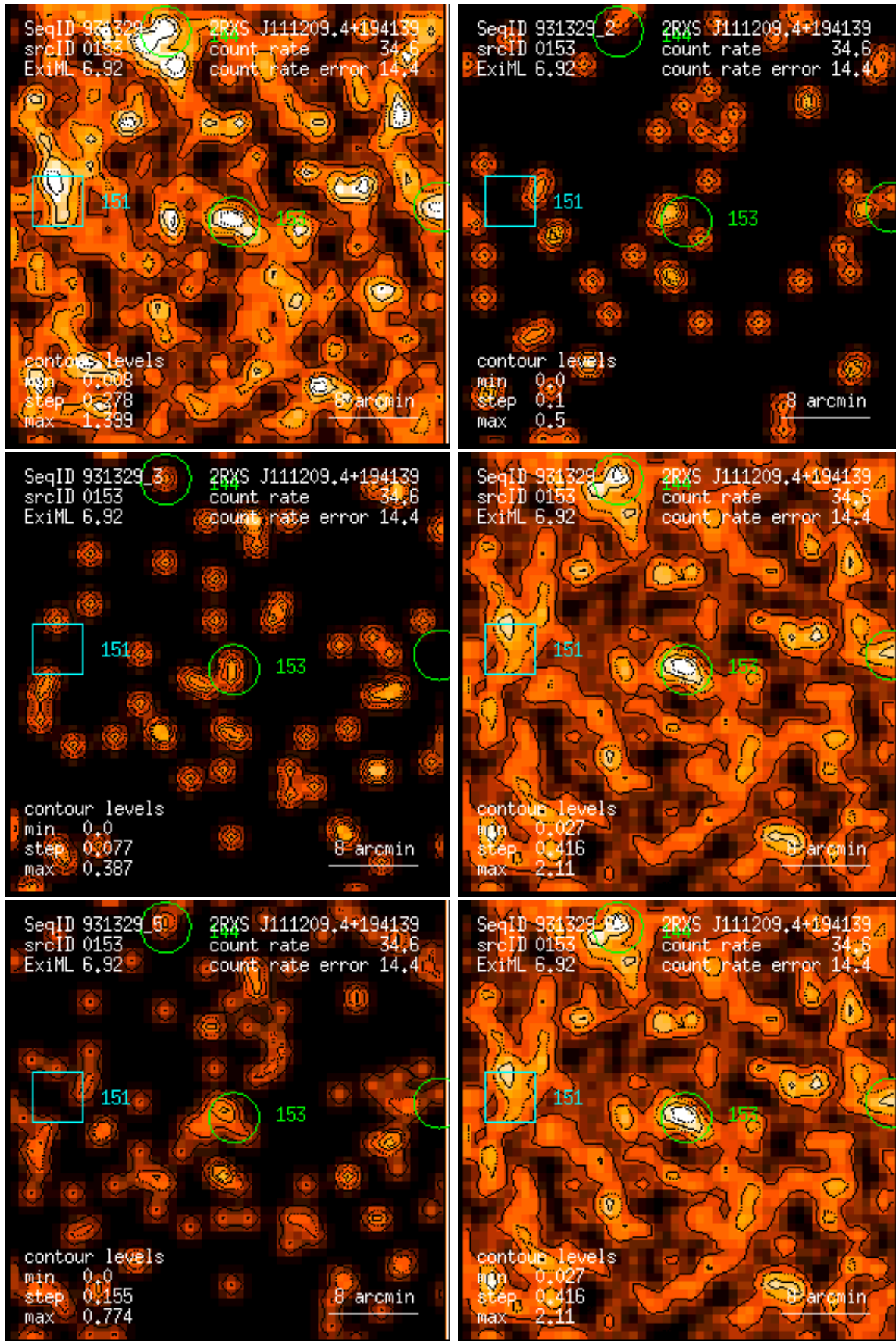
Figure 153: RASS 931329: detection 0153: band rate images, Gaussian filter: (1) PSPC channels 11 – 41, (2) 52 – 90, (3) 91 – 201, (4) 11 – 235, (5) 52 – 201, (6) 11 – 201. Broad band rates in counts/ks. Band rate contour levels in counts/ks/arcmin 2 .
