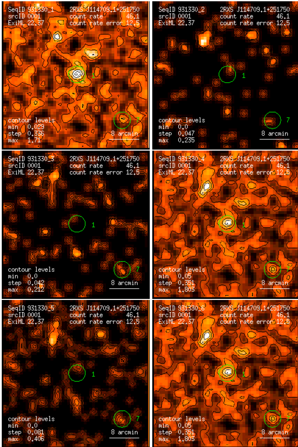
Figure 1: RASS 931330: detection 0001: band rate images, Gaussian filter: (1) PSPC channels 11 – 41, (2) 52 – 90, (3) 91 – 201, (4) 11 – 235, (5) 52 – 201, (6) 11 – 201. Broad band rates in counts/ks. Band rate contour levels in counts/ks/arcmin 2 .
