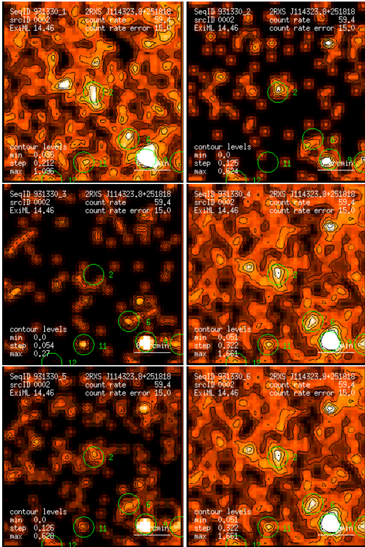
Figure 2: RASS 931330: detection 0002: band rate images, Gaussian filter: (1) PSPC channels 11 – 41, (2) 52 – 90, (3) 91 – 201, (4) 11 – 235, (5) 52 – 201, (6) 11 – 201. Broad band rates in counts/ks. Band rate contour levels in counts/ks/arcmin 2 .
