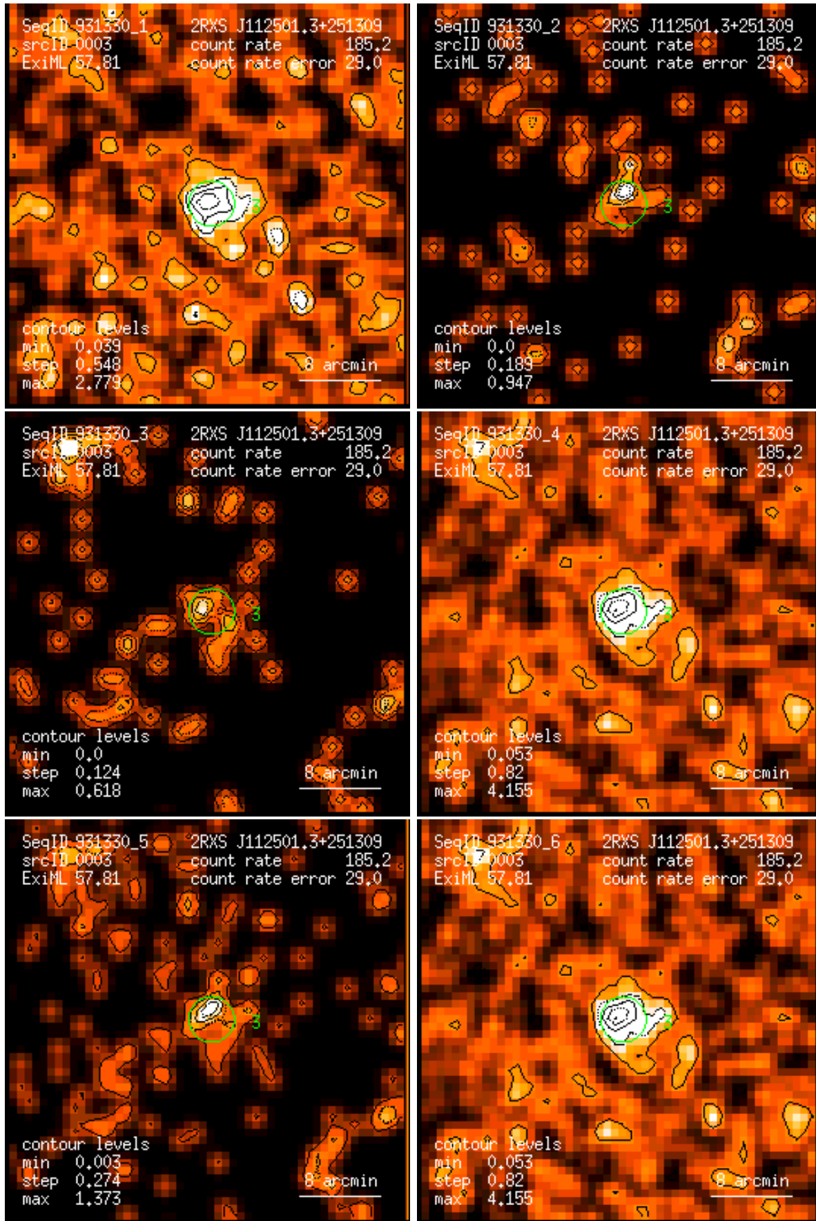
Figure 3: RASS 931330: detection 0003: band rate images, Gaussian filter: (1) PSPC channels 11 – 41, (2) 52 – 90, (3) 91 – 201, (4) 11 – 235, (5) 52 – 201, (6) 11 – 201. Broad band rates in counts/ks. Band rate contour levels in counts/ks/arcmin 2 .
